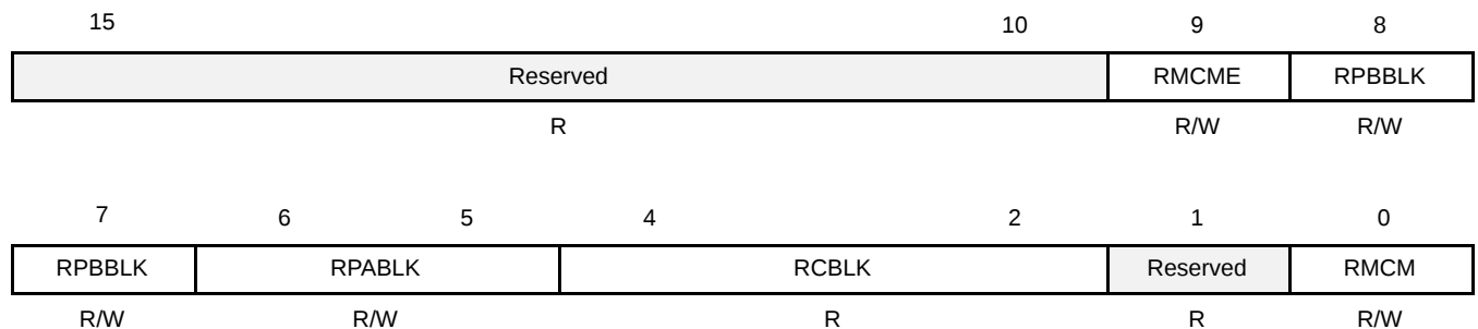
Figure 3–13. Multichannel Control Register (MCR2)
