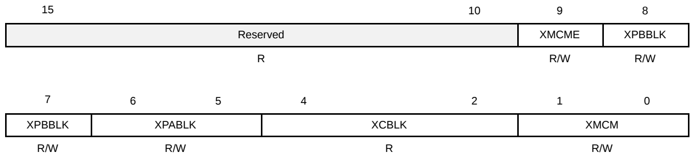
Figure 3–12. Multichannel Control Register (MCR1)
