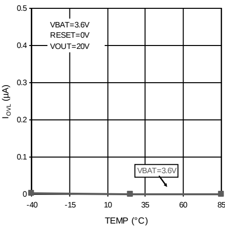
Figure 34. VOUT Leak Current vs Temperature
