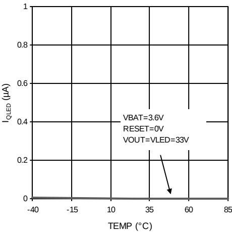
Figure 36. LED1, LED2 Leak Current vs Temperature
