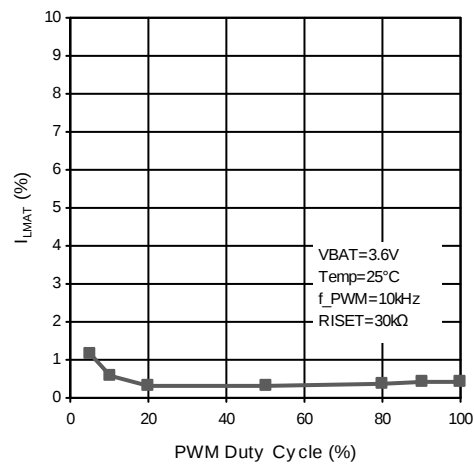
Figure 38. LED Current Matching vs PWM Duty (PWM output mode)
