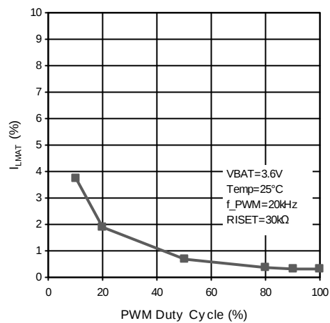
Figure 40. LED Current Matching vs PWM Duty (DC output mode)
