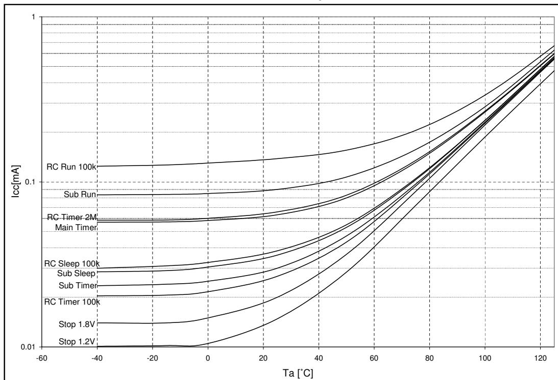
MB96F346/F347/F348Y/R/A Low power mode currents
