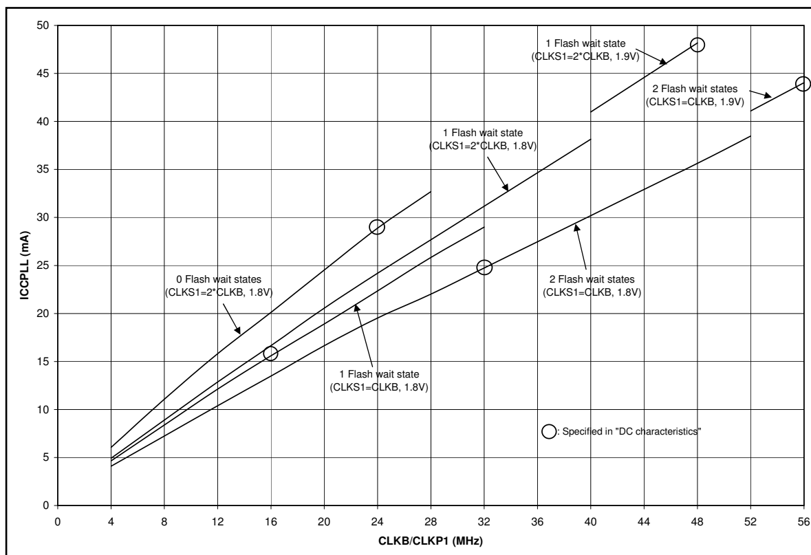
MB96F348T/H/C PLL Run mode currents
