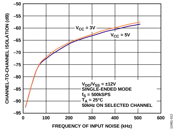
Figure 14. Channel-to-Channel Isolation
