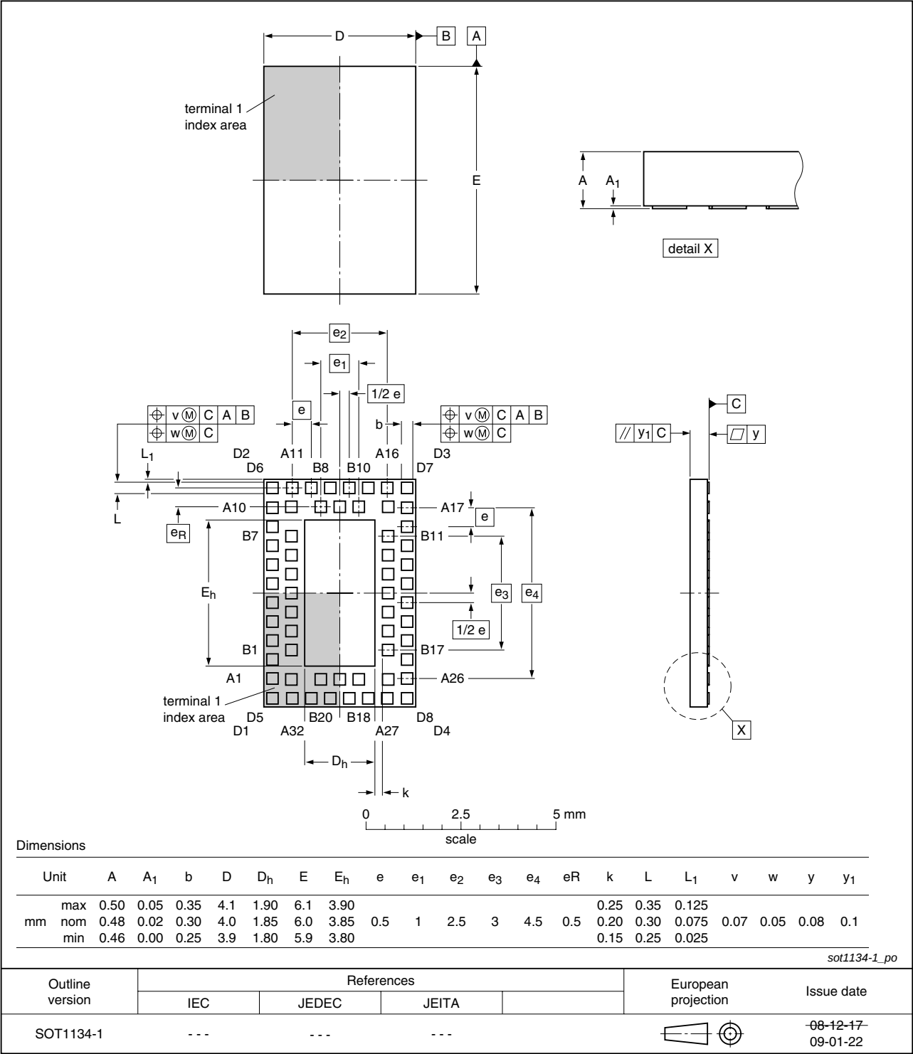
Fig 12. Package outline SOT1134-1 (HXQFN60U)
