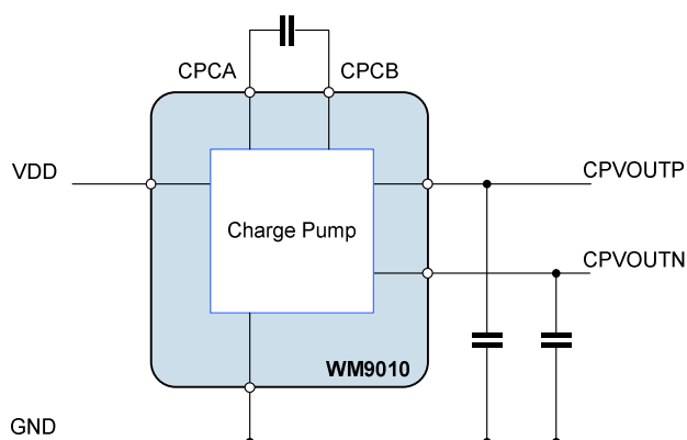
Figure 2 External Connections for Charge Pump
