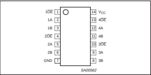
Figure 1. SO14, SSOP14, and TSSOP14
