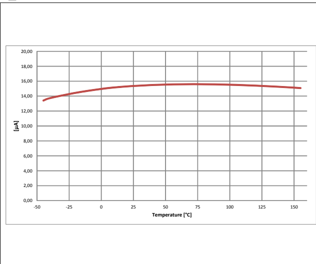
Input Current High Level
