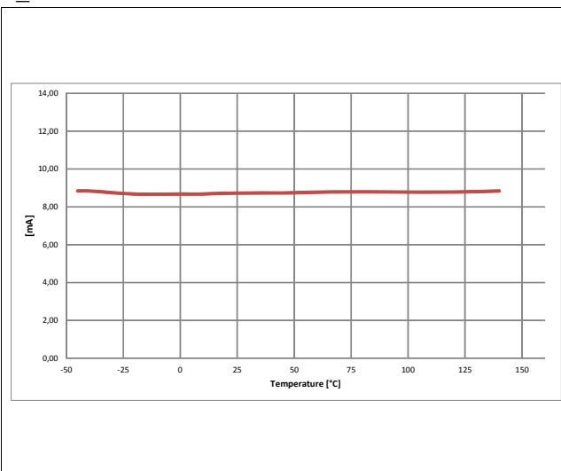
Open Load Detection ON State Threshold
