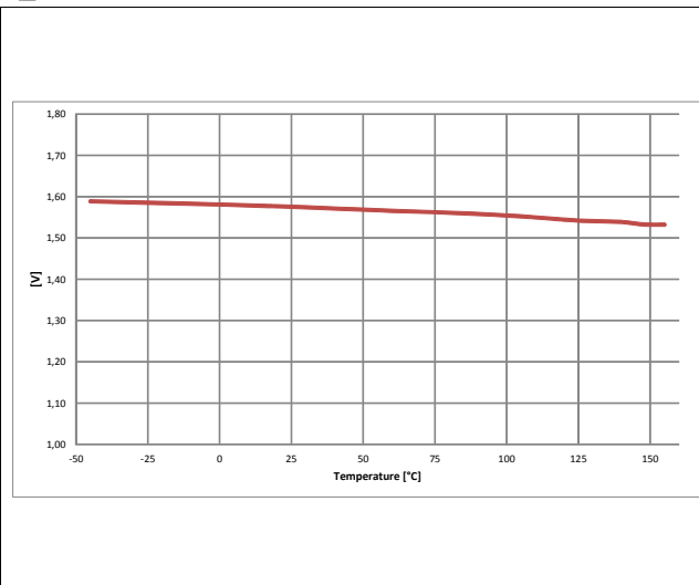
Input Voltage Threshold
