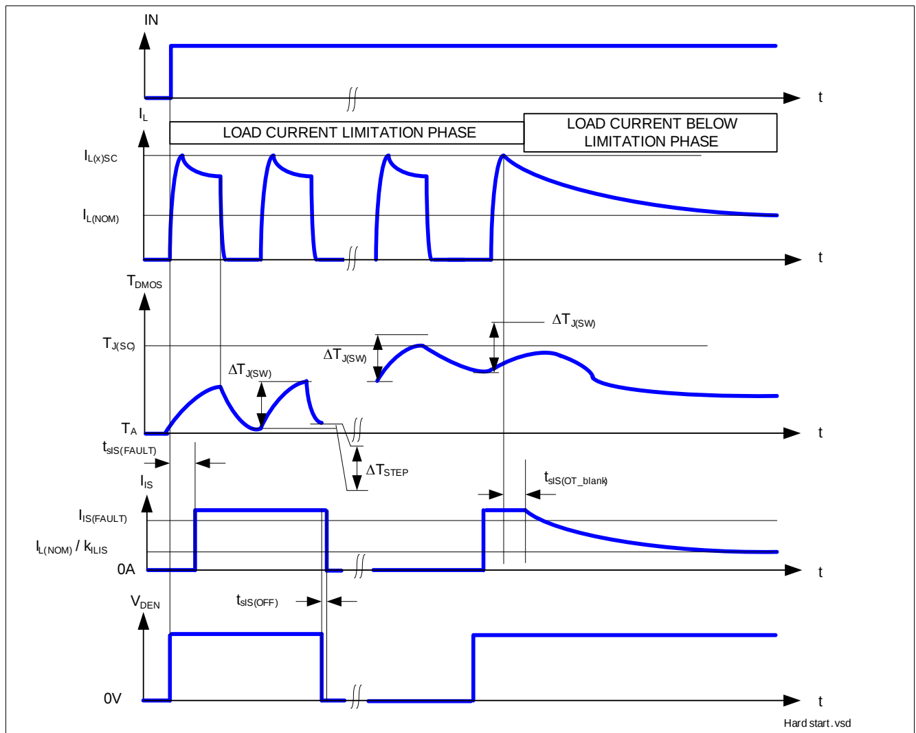
Figure 16 Overload Protection
