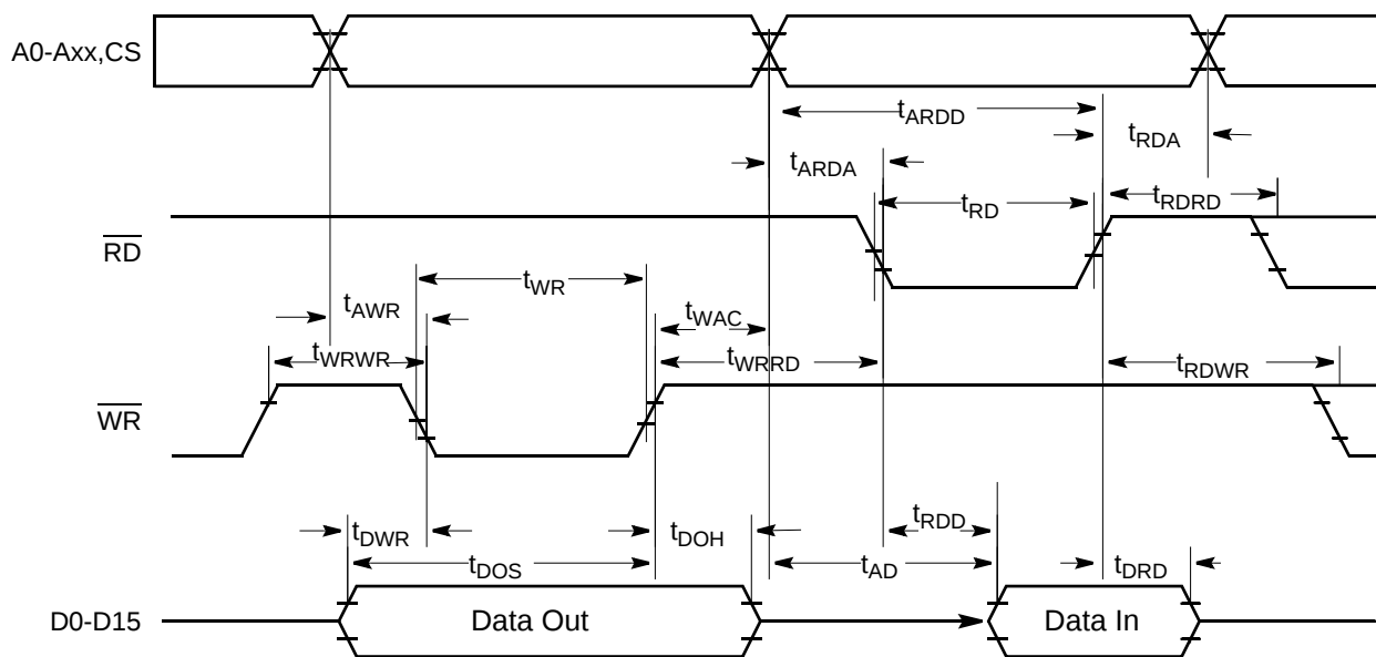
Figure 10-4 External Memory Interface Timing
