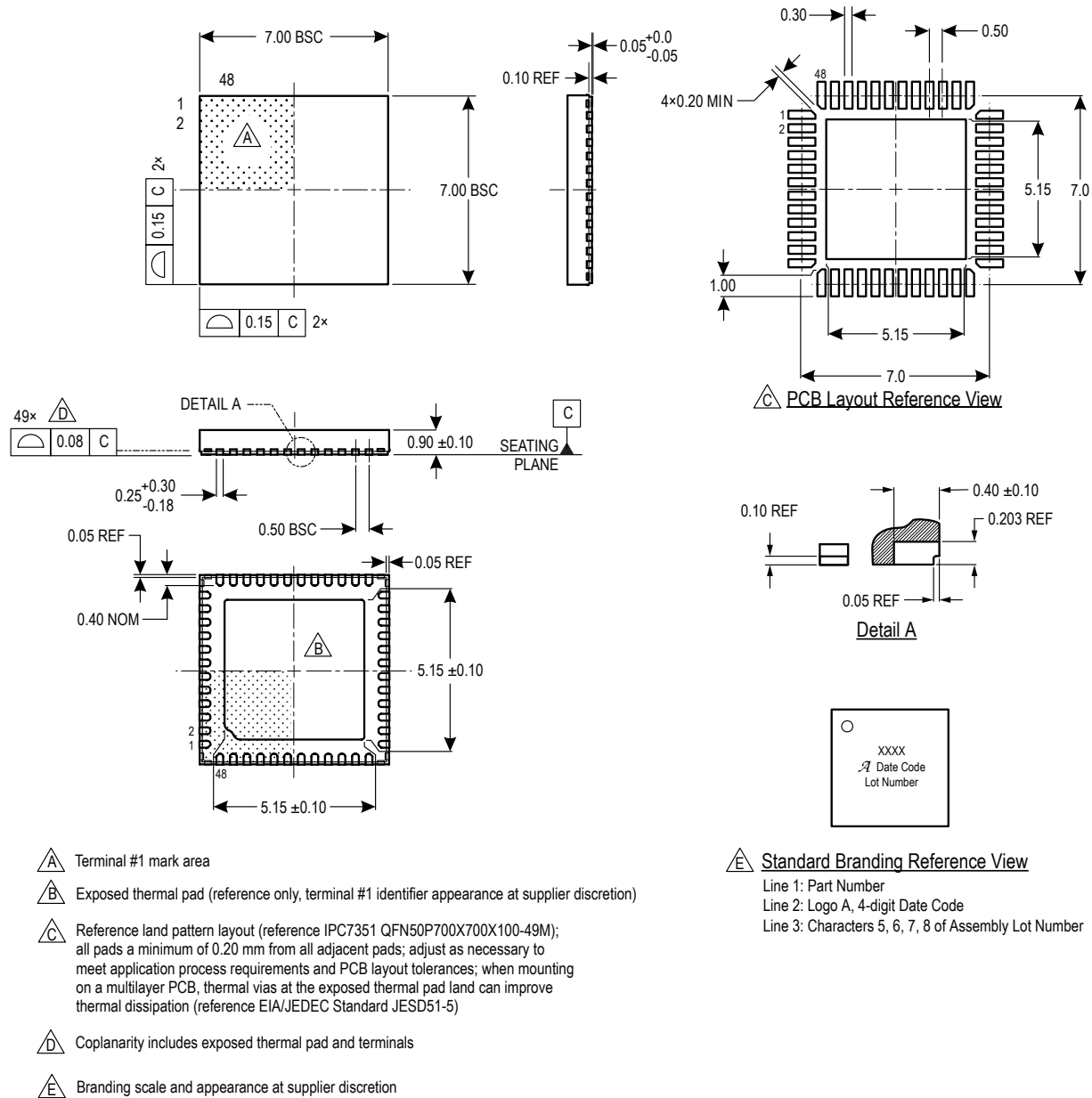
Figure 49: Package EV, 48-Pin 7 mm × 7 mm QFN with Exposed Thermal Pad and Wettable Flank
