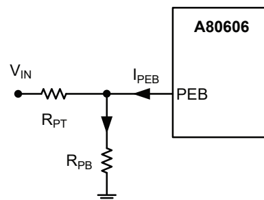
Figure 23: PEB delay setup circuit with connection to V_{IN}
