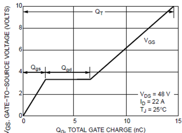
Figure 59: Gate Charge vs. Gate-Source Voltage chart for a suitable MOSFET (NVD5867NL). Note that its plateau is at ~3.5 V, and its total gate charge is about 10 nC as V_{GS} ramps up from 0 to 6.5 V.
