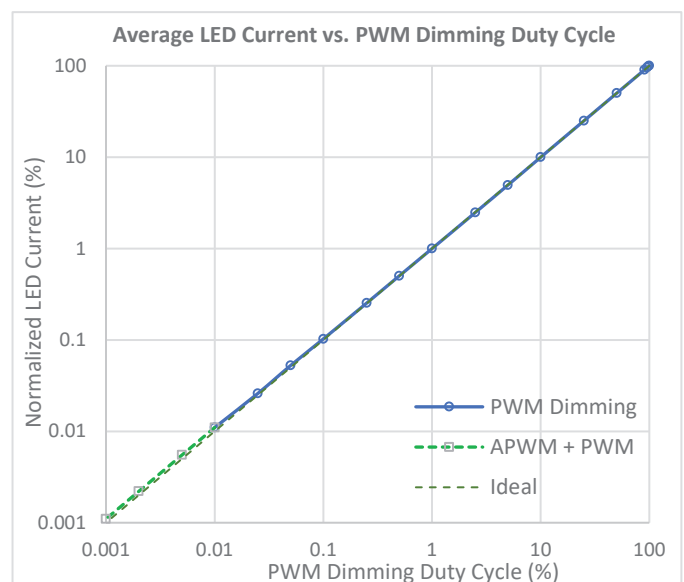
Figure 29: How to achieve 100,000:1 dimming ratio by using both PWM and APWM. Test conditions: V_{IN} = 12 \text{ V} , V_{OUT} = 25 \text{ V} ( 8 \times WLED ), total LED current = 400 mA, PWM frequency = 200 Hz, APWM frequency = 100 kHz.
