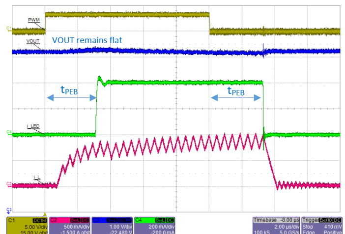
Figure 21: A80606 PWM dimming operation with PEB delay set to 3 µs. Note that V_{OUT} ripple is reduced to ~0.2 V.
