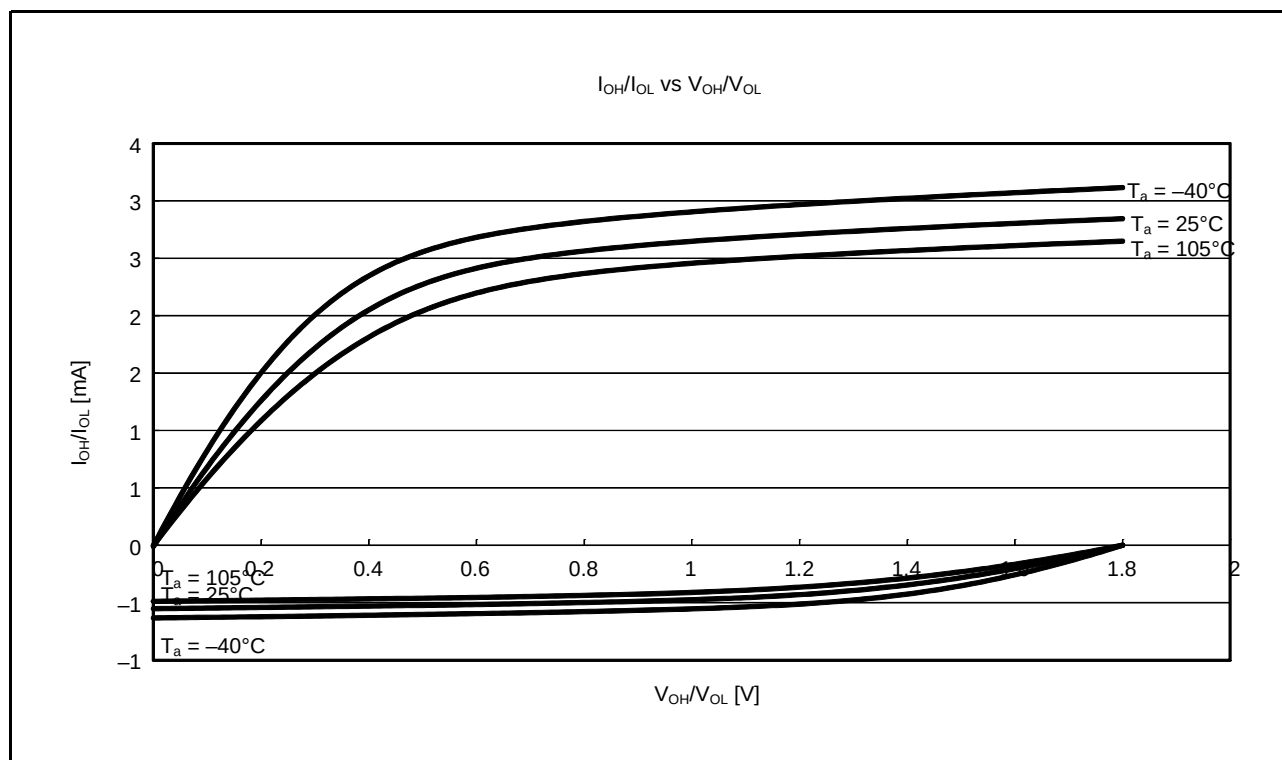
Figure 5.15 V_{OH}/V_{OL} and I_{OH}/I_{OL} Temperature Characteristics of Ports P40 to P44, P46, Ports P90 to P92, Ports PJ6, PJ7 at V_{CC} = 1.8\text{ V} (Reference Data)
