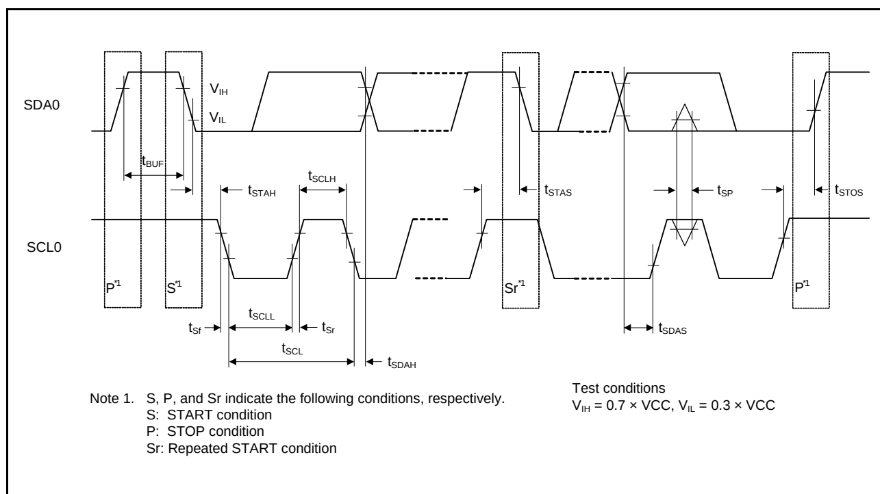
Figure 5.49 IIC Bus Interface Input/Output Timing and Simple I²C Bus Interface Input/Output Timing
