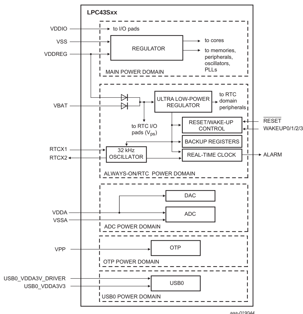
Fig 8. Power domains
