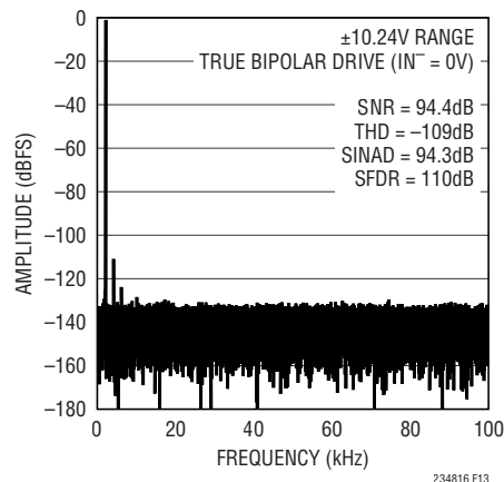
Figure 13. 32k Point FFT f_{\text{SMPL}} = 200\text{ksps} , f_{\text{IN}} = 2\text{kHz}
