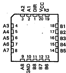
SN54HC' ... FK PACKAGE
