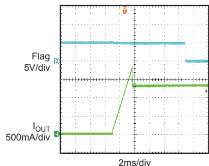
Ramped Load on Enabled Device
