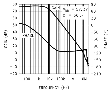
Amplifier Open Loop Frequency Response
