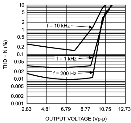
THD+N vs Output Voltage V_{DD} = 3V , Z_L = 2\mu F + 30\Omega , V_1 = 5.0V
