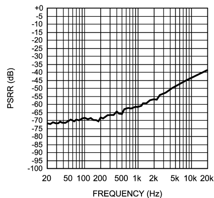
PSRR vs Frequency V_1 = 5.8V , Z_L = 2\mu F + 30\Omega , V_{ripple} = 200mV_{pp} , A_{V-BTL} = 26dB
