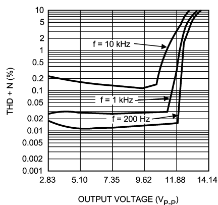
THD+N vs Output Voltage V_{DD} = 4.2V , Z_L = 2\mu F + 30\Omega , V_1 = 6.1V
