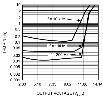
THD+N vs Output Voltage V_{DD} = 3V , Z_L = 2\mu F + 30\Omega , V_1 = 6.1V
