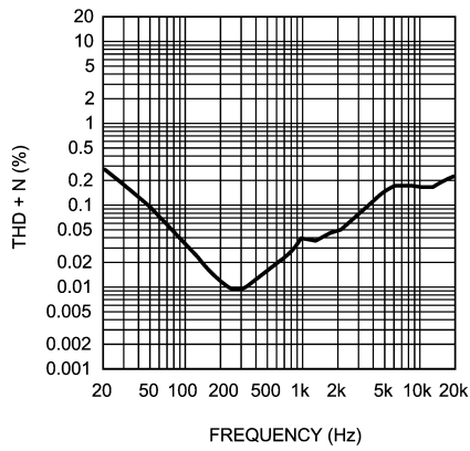
THD+N vs Frequency V_{DD} = 3V , Z_L = 2\mu F + 30\Omega , V_{OUT} = 10V_{P-P}
