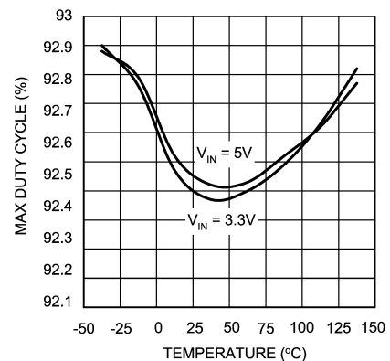
Max. Duty Cycle vs Temperature - "X"
