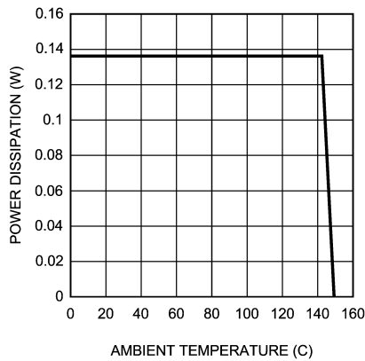
Power Derating Curve - LLP P_{DMAX} = 136mW V_{DD} = 4.2V , Z_L = 2\mu F + 30\Omega
