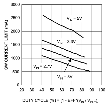
Switch Current Limit vs Duty Cycle - "X"
