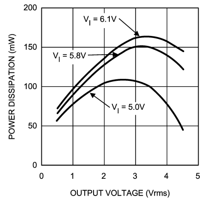
Power Dissipation vs Output Voltage V_{DD} = 3.0V , Z_L = 2\mu F + 30\Omega
