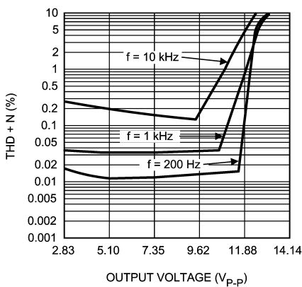
THD+N vs Output Voltage V_{DD} = 3V , Z_L = 2\mu F + 30\Omega , V_1 = 5.8V
