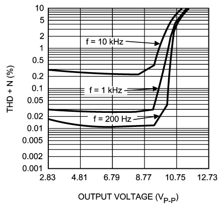
THD+N vs Output Voltage V_{DD} = 4.2V , Z_L = 2\mu F + 30\Omega , V_1 = 5.0V
