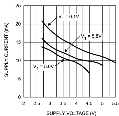
Supply Voltage vs Supply Current Z_L = 2\mu F + 30\Omega , V_{IN} = 0V
