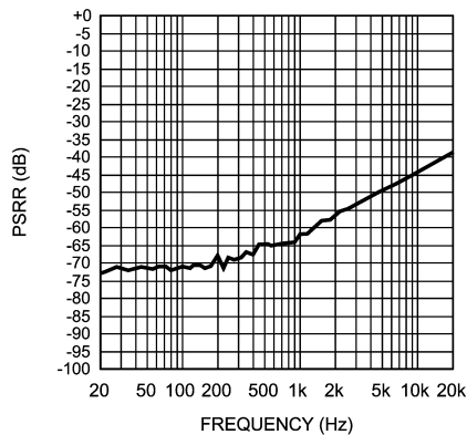
PSRR vs Frequency V_I = 6.1V , Z_L = 2\mu F + 30\Omega , V_{ripple} = 200mV_{pp} , A_{V-BTL} = 26dB
