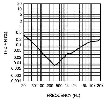
THD+N vs Frequency V_{DD} = 4.2V , Z_L = 2\mu F + 30\Omega , V_{OUT} = 10V_{P-P}
