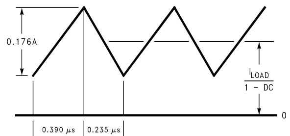
FIGURE 2. 10 \mu H Inductor Current 5V - 12V Boost (LM4802B)
