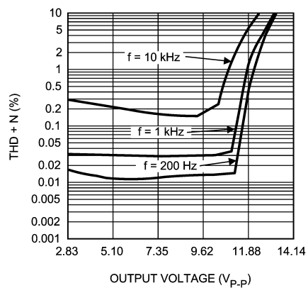
THD+N vs Output Voltage V_{DD} = 4.2V , Z_L = 2\mu F + 30\Omega , V_1 = 5.8V
