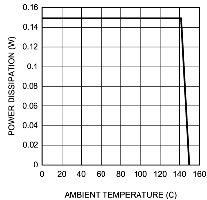
Power Derating Curve - LLP P_{DMAX} = 150mW V_{DD} = 3.0V , Z_L = 2\mu F + 30\Omega
