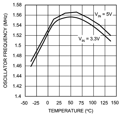
Oscillator Frequency vs Temperature - "X"
