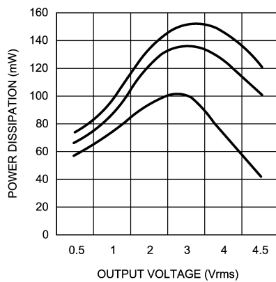
Power Dissipation vs Output Voltage V_{DD} = 4.2V , Z_L = 2\mu F + 30\Omega From top to bottom: V_I = 6.1V , V_I = 5.8V , V_I = 5.0V
