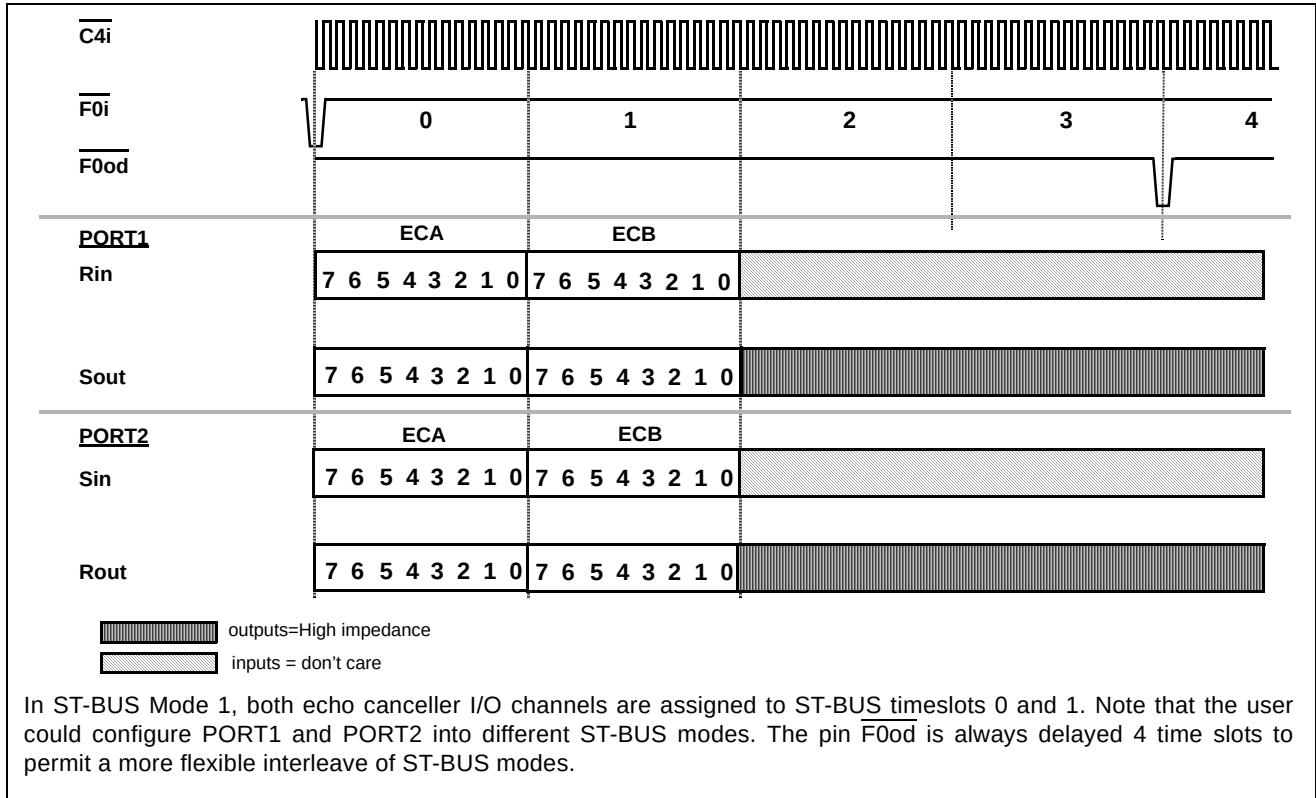
Figure 5 - ST-BUS 8 Bit Companded PCM I/O on Timeslots 0 &amp; 1 (Mode 1)
