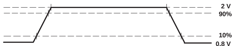
Figure 5. TTL-Level Inputs
