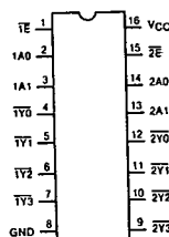
TERMINAL ASSIGNMENT
