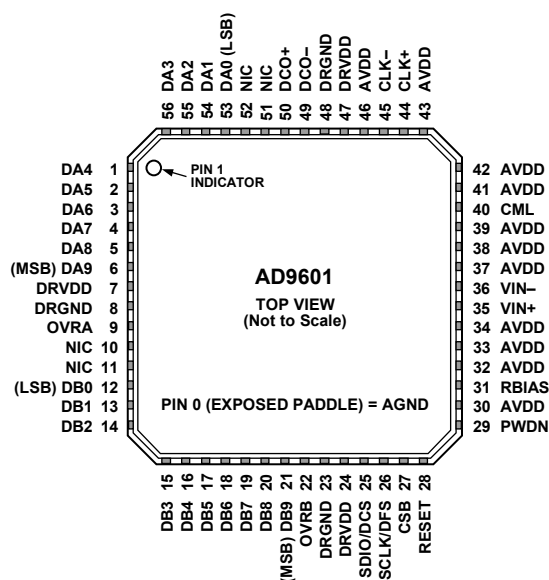
Figure 4. Pin Configuration
