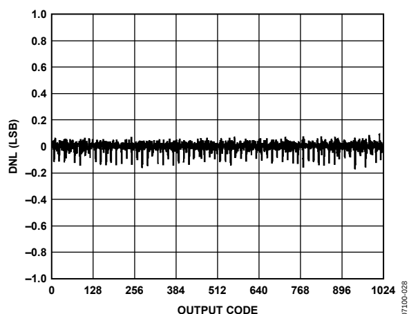
Figure 19. AD9601-200 DNL; 200 MSPS
