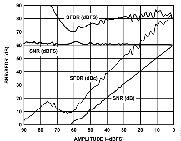
Figure 16. AD9601-200 SNR/SFDR vs. Input Amplitude; 170.3 MHz
