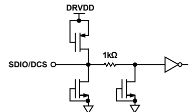
Figure 10. Equivalent SDIO/DCS Input Circuit
