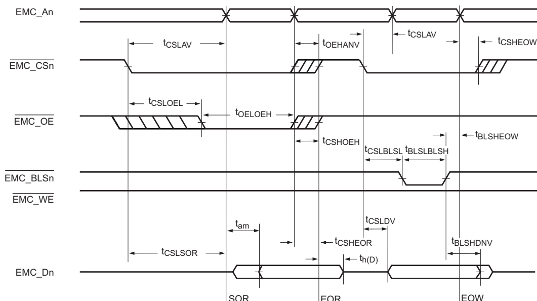
Fig 31. External static memory read/write access (PB = 0)
