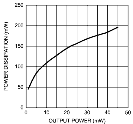
Power Dissipation vs Output Power V_{DD} = 3.3V , R_L = 32\Omega , f = 1kHz Mode 2, 4, 6, OCL
