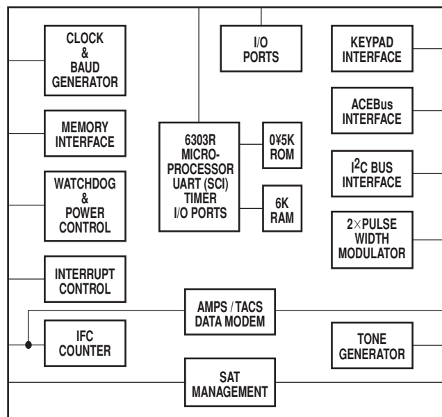
Figure 2 - ACE9050 simplified block diagram
