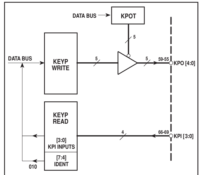
Figure 25 - Keyport configuration
