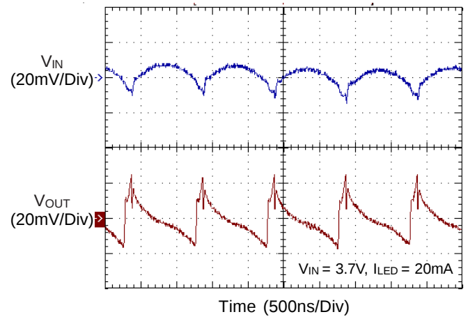
Ripple Voltage
