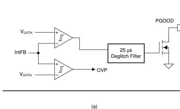
Figure 8-5. Power Good Monitor (a) Boost configuration
