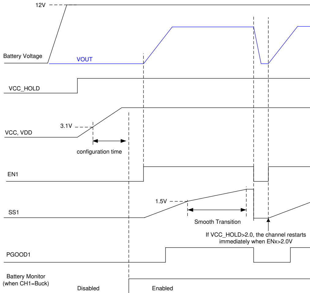
Figure 8-12. Start-up Sequence ( V_{CC\_HOLD} > 2.0\text{ V} , CH1 = Buck)
