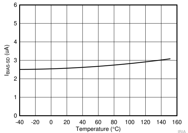
Figure 7-10. I_{BIAS-SD} vs Temperature
