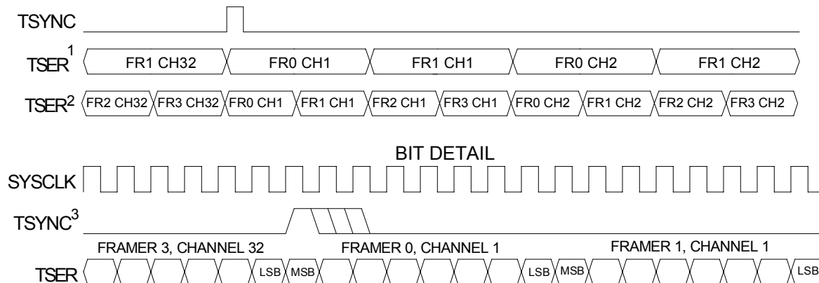
Figure 24-7. Transmit Interleave Bus Operation
