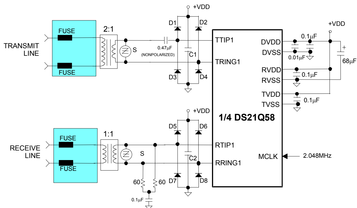
Figure 21-3. External Analog Connections (Protected Interface)
