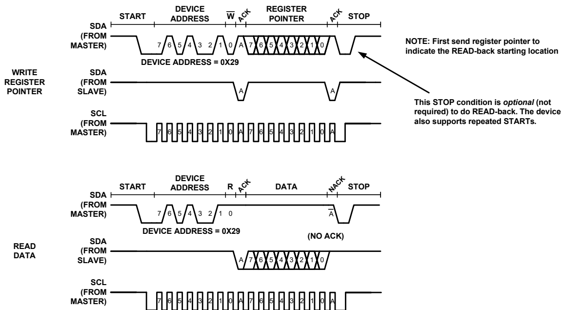
FIGURE 47. I 2 C READ TIMING DIAGRAM
