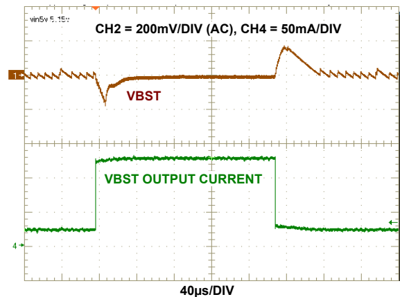
FIGURE 7. V_{BST} LOAD TRANSIENT, V_{BST} = 5.15\text{V}
