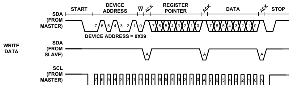
FIGURE 46. I 2 C WRITE TIMING DIAGRAM
