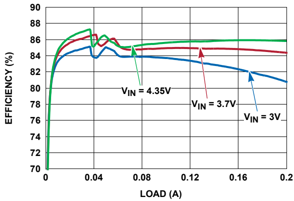
FIGURE 4. DISPLAY POWER SYSTEM EFFICIENCY, V_P/V_N = \pm 5\text{V}
