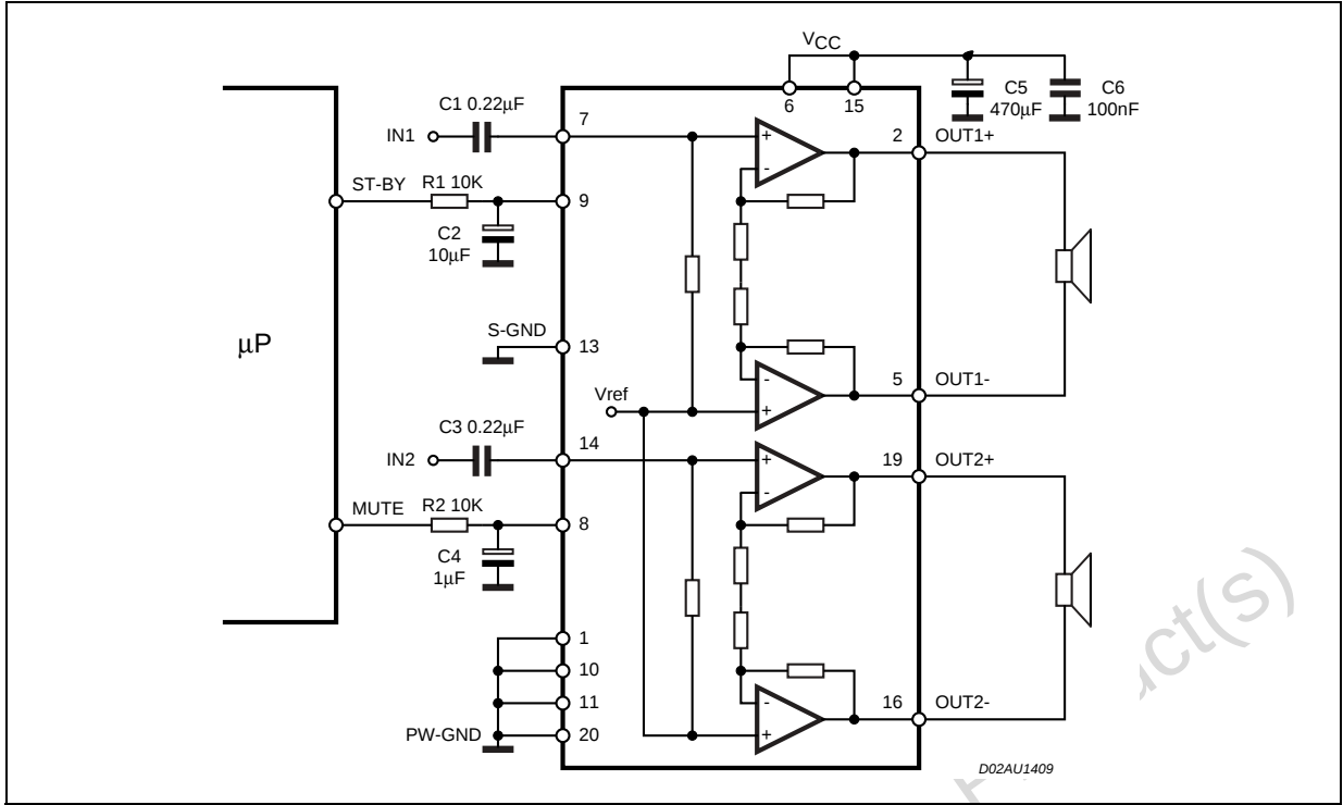
Figure 4. Microprocessor Application
