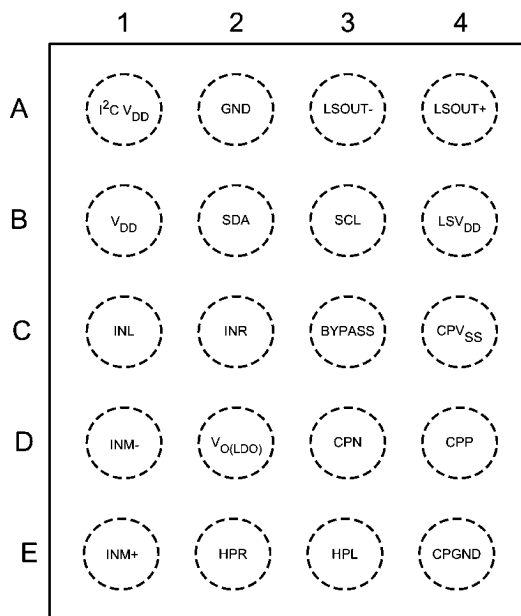
Top View (Bump Side Down) (See NS Package Number TLA20KGA)
