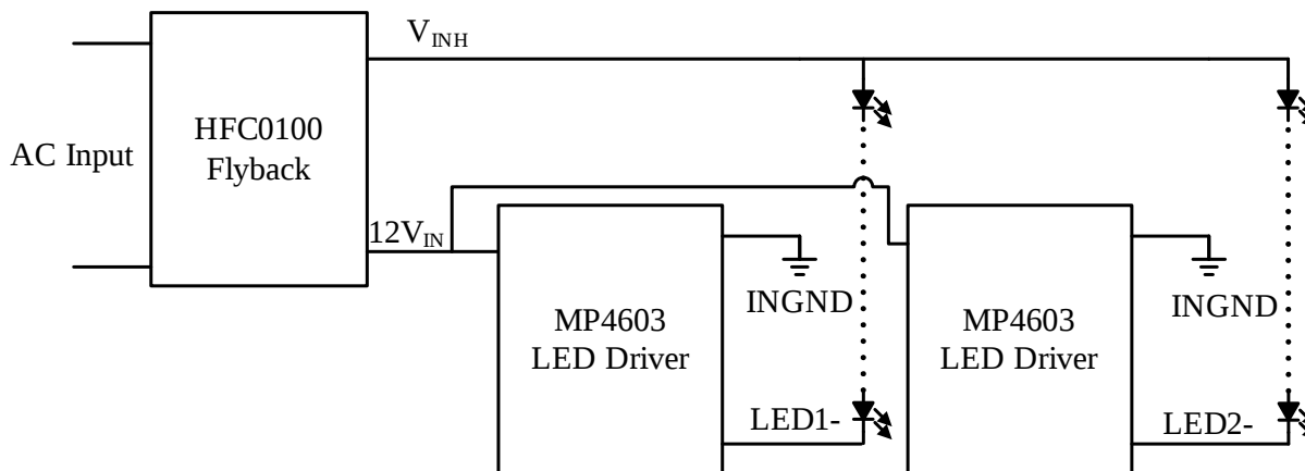
Figure 4: System Power Block Diagram
