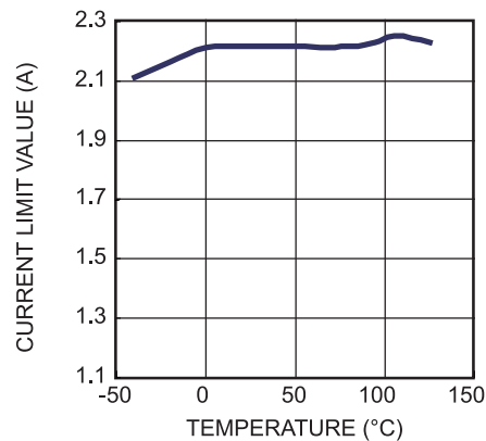
Current Limit Value vs. T_J
