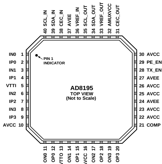
Figure 3. Pin Configuration
