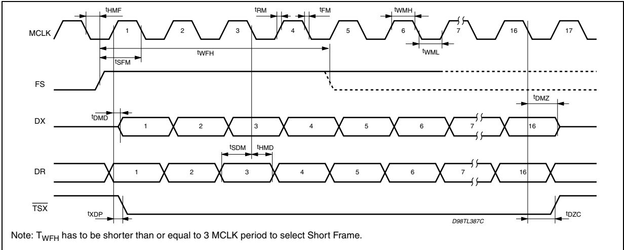
Figure 9. Pin-strap mode long frame sync. timing
