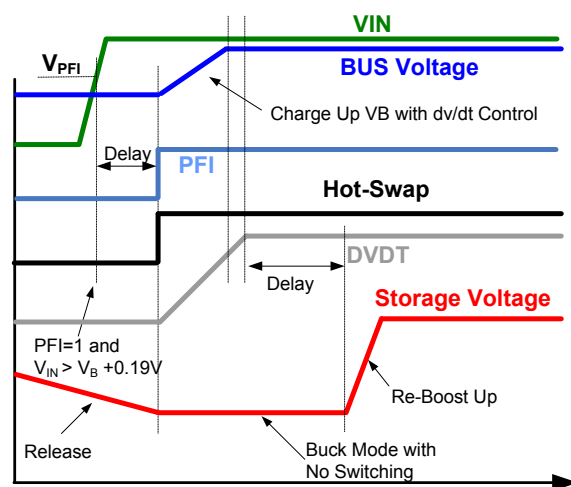
Figure 4: Re-Charge Sequence
