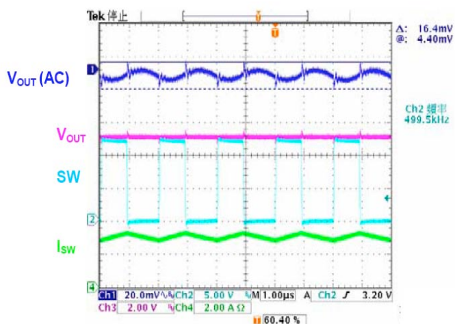
Figure 8. Output Ripple ( V_{IN}=12V , V_{OUT}=5V , I_{OUT}=3A )
