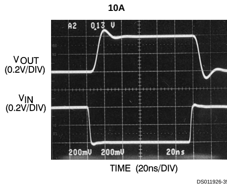
FIGURE 10. Resistive Isolation of C_L Provides Higher Fidelity Pulse Response. R_f and R_s Could Also Be Increased to Maintain A_v = -1 and Improve Pulse Response Characteristics.
