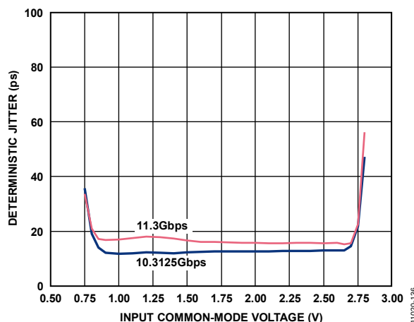
Figure 23. Deterministic Jitter vs. Input Common-Mode Voltage
