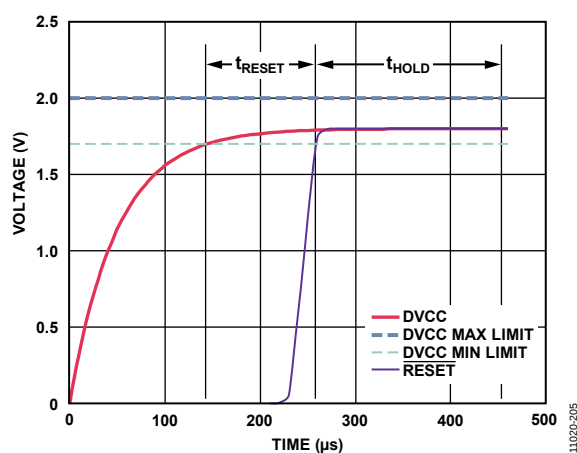
Figure 5. RESET Timing Diagram
