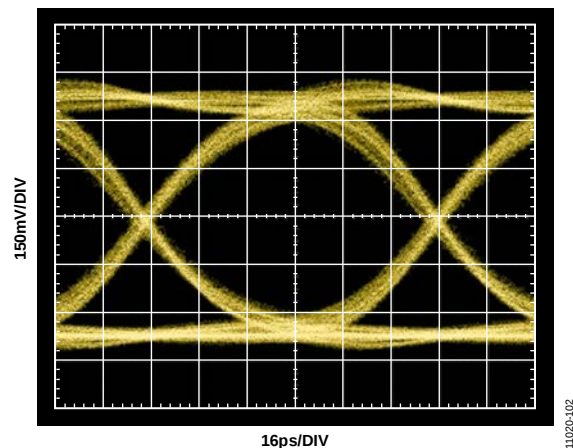
Figure 29. 10.3125 Gbps Output Eye (TP2 from Figure 47)
