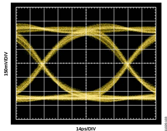
Figure 30. 11.3 Gbps Output Eye (TP2 from Figure 47)
