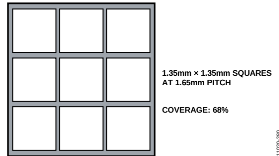
Figure 77. Typical Thermal Pad Stencil Design
