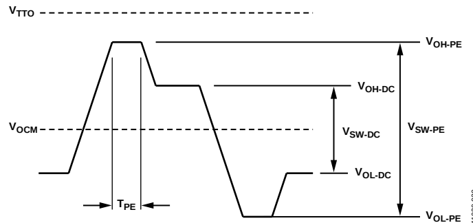
Figure 61. Step Response of Two-Tap FFE
