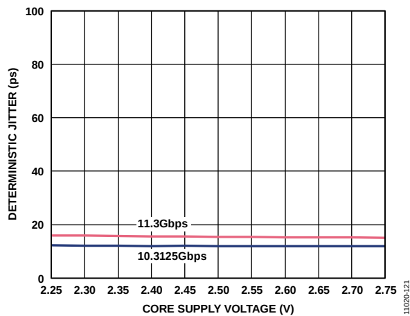
Figure 8. Deterministic Jitter vs. Core Supply Voltage ( V_{CC} )
