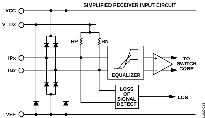
Figure 51. Simplified Input Circuit
