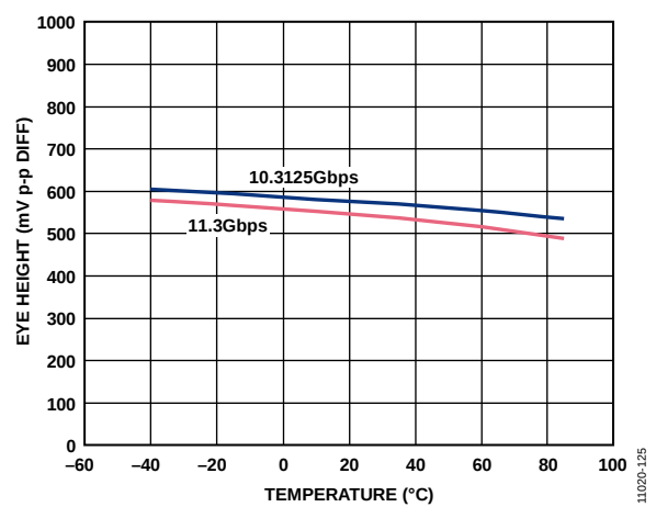
Figure 12. Eye Height vs. Temperature
