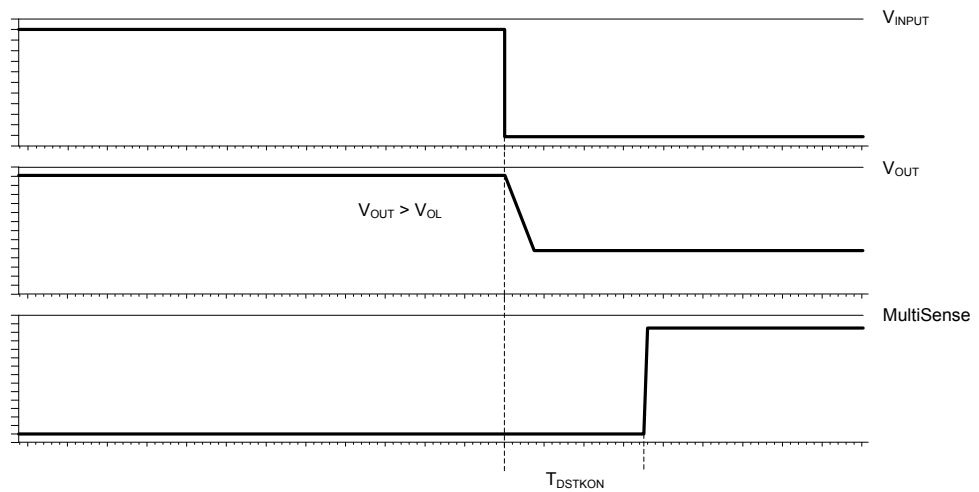
Figure 8. T_{\text{DSTKON}}
