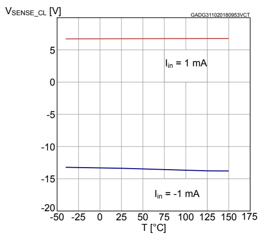
Figure 32. V_{\text{SENSE\_CLAMP}} vs. T_{\text{case}}
