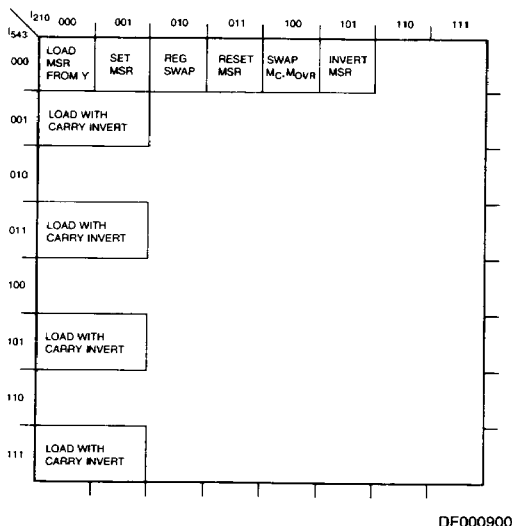
MAP 2. MACHINE STATUS REGISTER INSTRUCTION CODES
