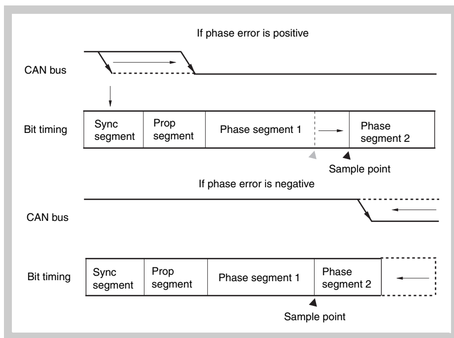
Figure 20-21 Resynchronization
