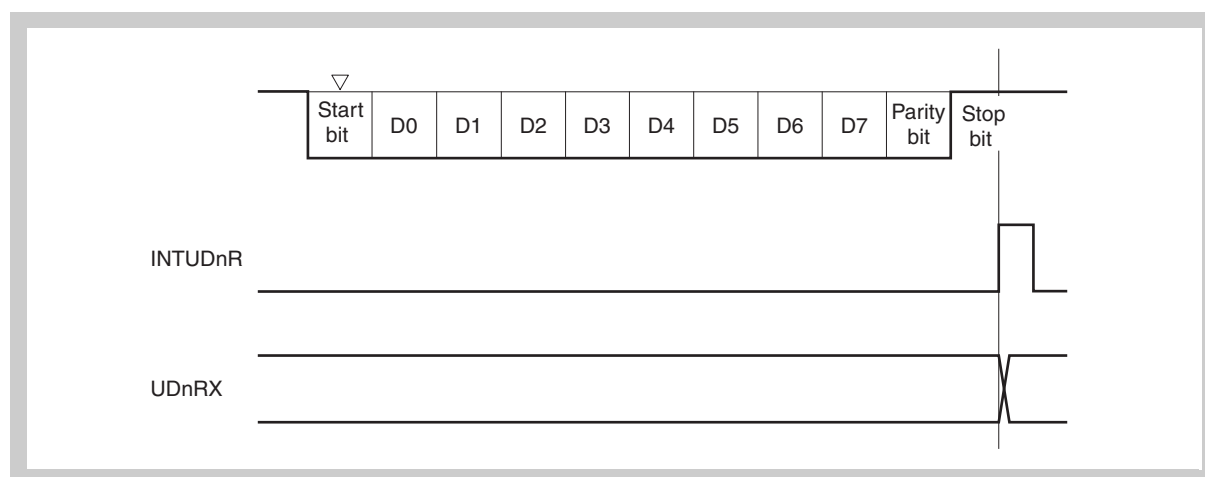
Figure 17-8 UART reception
