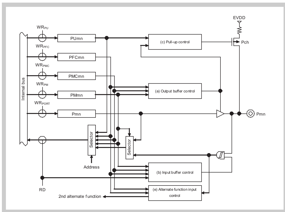
Figure 2-28 Port type Ex1-U block diagram
