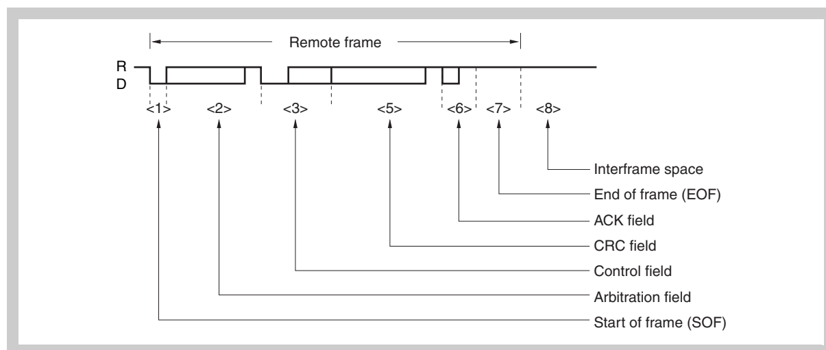
Figure 20-4 Remote frame
