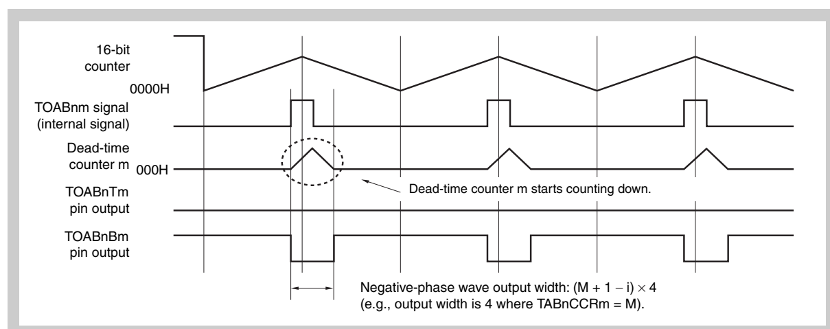
Figure 22-17 Operation of Dead-Time Counter m (1) In vicinity of 0% output (TABnCCRM register = i \geq M + 1 - a/2 , TABnCCR0 register = M, TABnDTC register = a)
