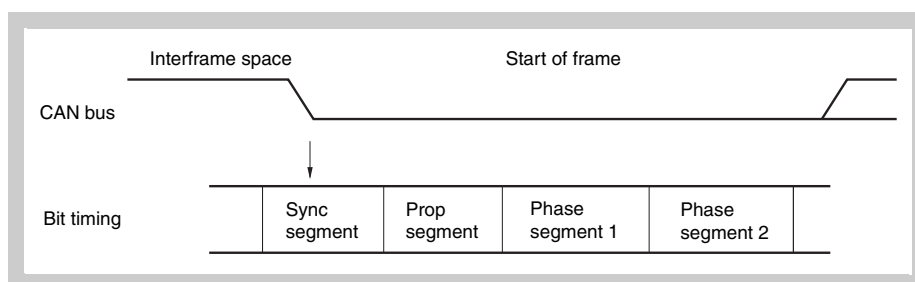
Figure 20-20 Adjusting synchronization of data bit
