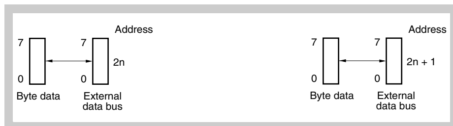
Figure 9-13 Left: Access to even address ( 2n ) Right: Access to odd address ( 2n + 1 )
