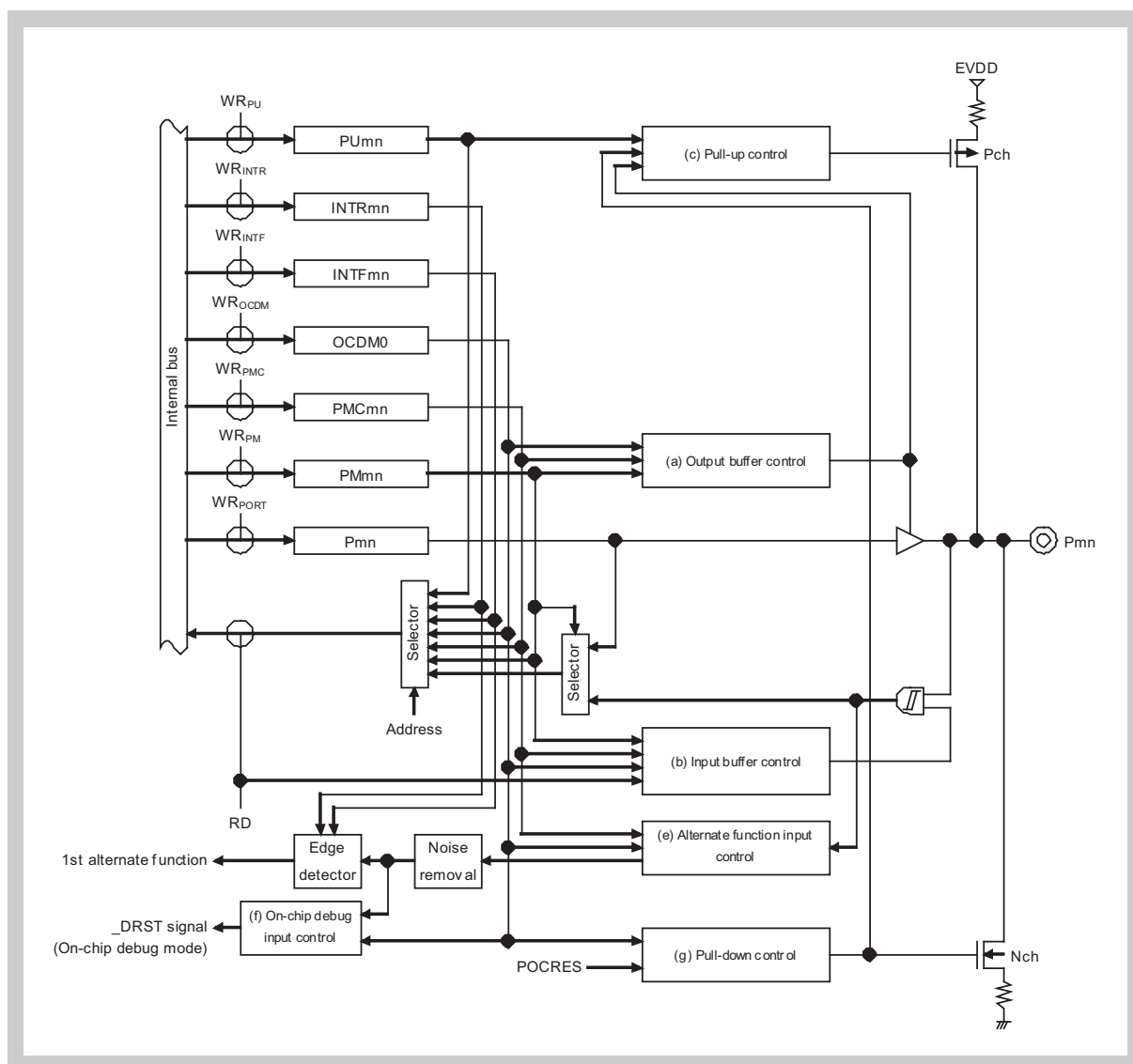
Figure 2-19 Port type D1O1-UI block diagram
