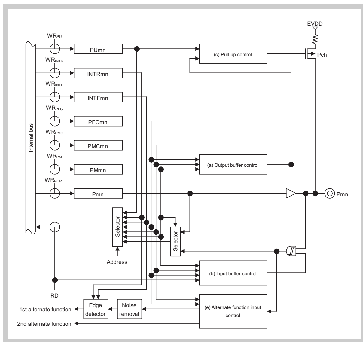
Figure 2-25 Port type E11-UI block diagram
