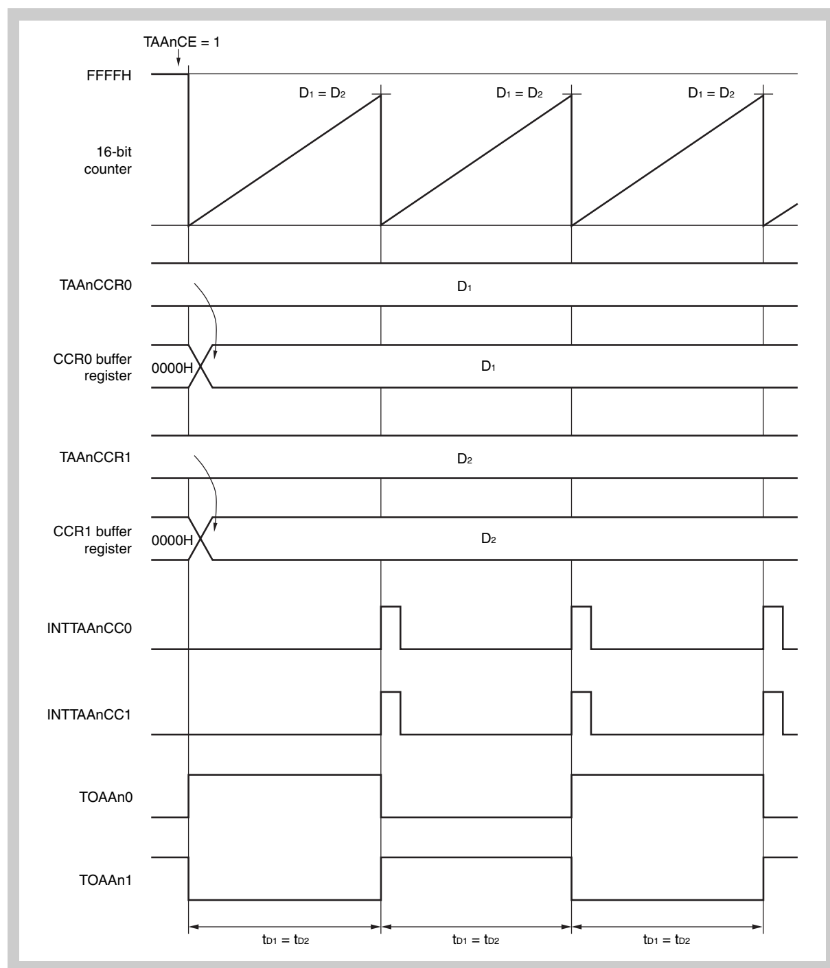
Figure 11-12 Basic operation timing in interval timer mode when D1 = D2 ; TAAAnCCR0 and TAAAnCCR1 are not rewritten, and TOAAAn0 and TOAAAn1 are output (TAAAnOE0 = 1, TAAAnOE1 = 1, TAAAnOL0 = 0, TAAAnOL1 = 1)
