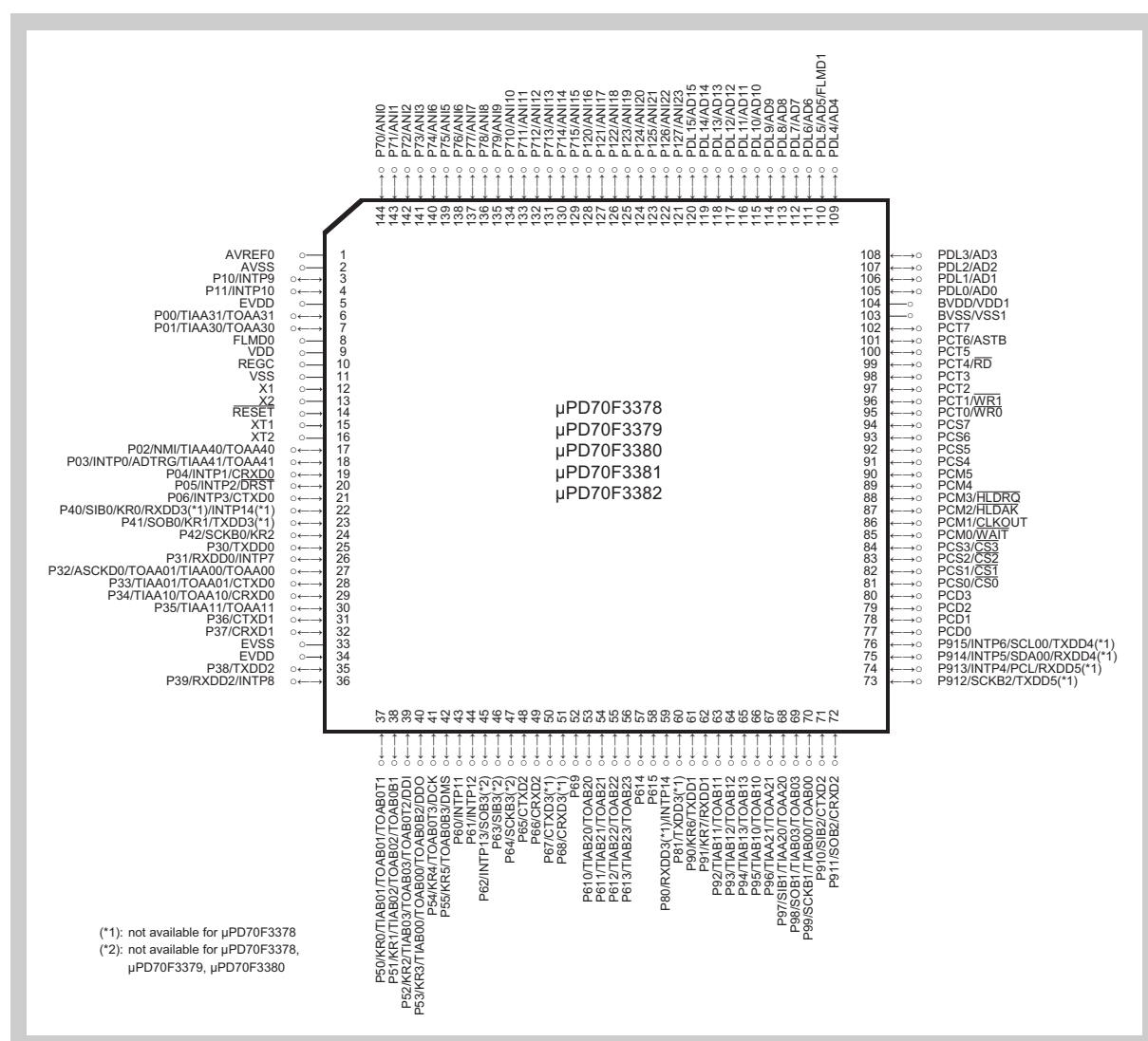
Figure 2-63 V850ES/FJ3 package pin assignment
