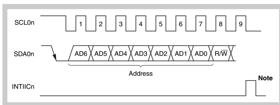
Figure 19-7 Address
