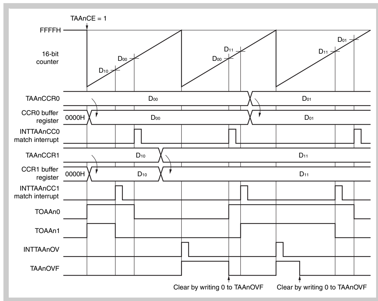
Figure 11-26 Basic Operation Timing in Free-Running Mode (TAA n CCS1 = 0, TAA n CCS0 = 0) (TAA n OEm = 1, TAA n OEL = 1, TAA n OL0 = 0, TAA n OL1 = 0)
