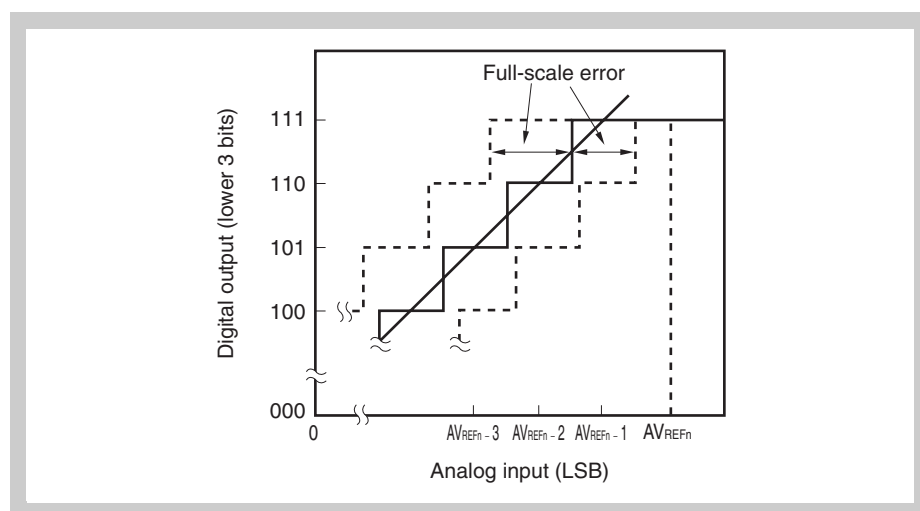
Figure 21-17 Full-scale error
