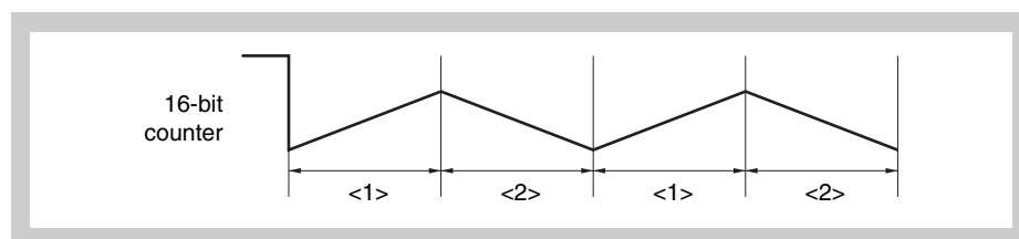
Figure 22-31 Example of Rewriting TABnCCR0 Register
