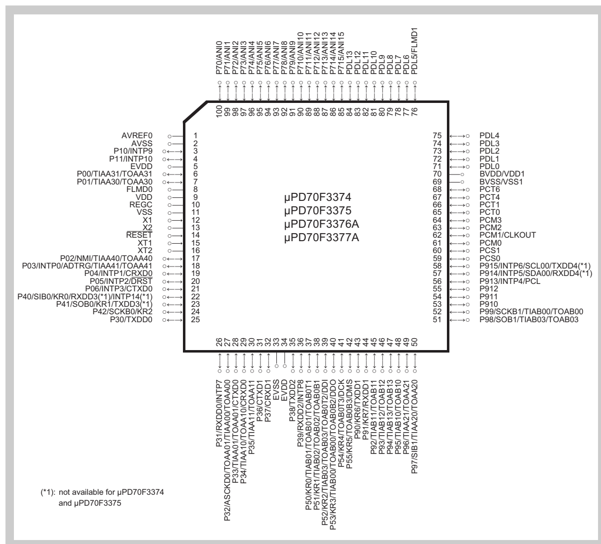
Figure 2-62 V850ES/FG3 package pin assignment
