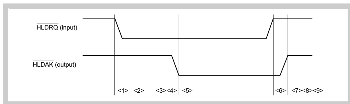
Figure 9-5 Bus hold state transition
