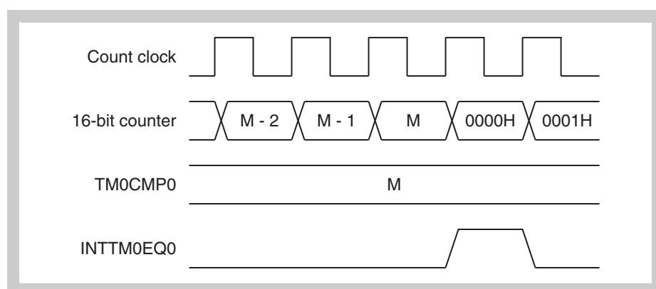
Figure 13-2 Timing of operation in interval timer mode
