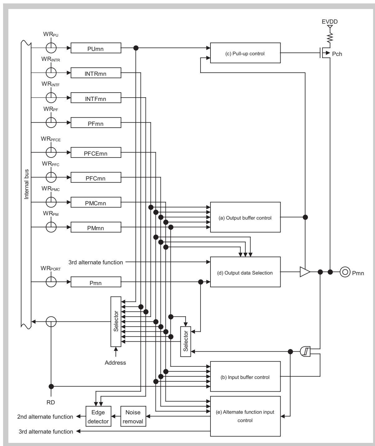
Figure 2-52 Port type Fx12x-UF1 block diagram
