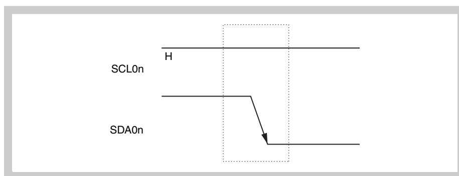
Figure 19-6 Start condition
