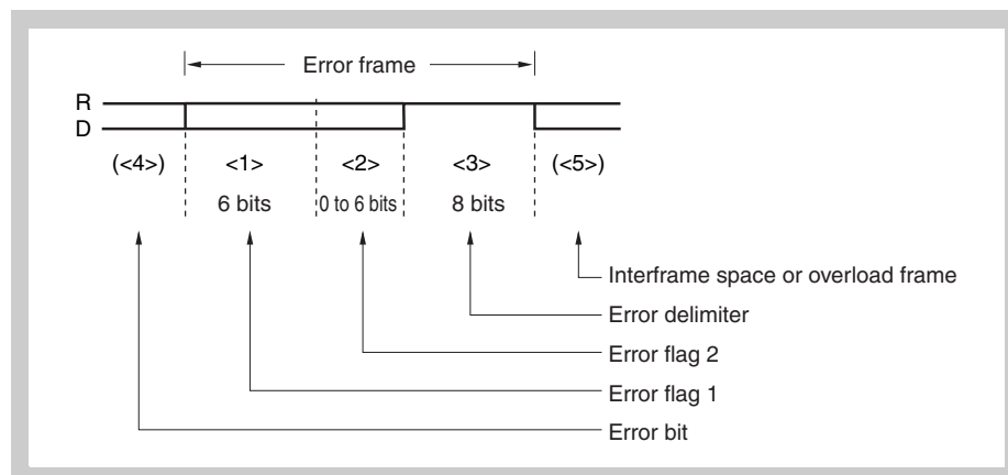
Figure 20-15 Error frame
