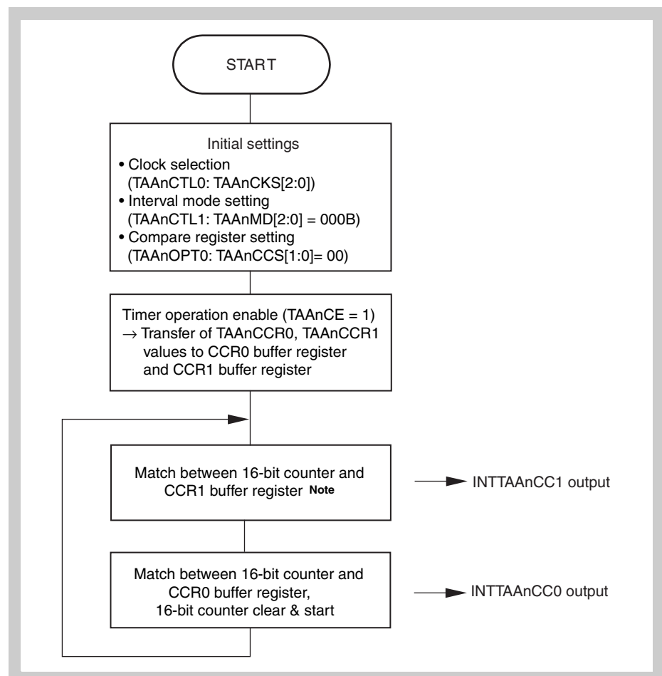
Figure 11-10 Flowchart of basic operation in interval timer mode
