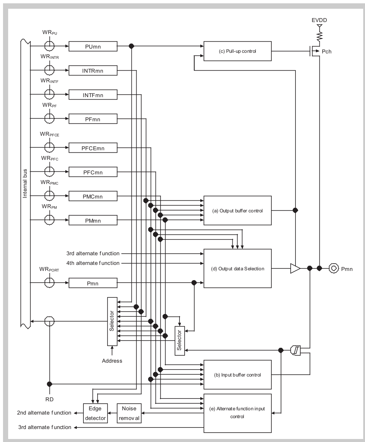
Figure 2-50 Port type Fx120-UF1 block diagram
