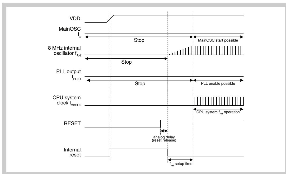
Figure 26-3 CPU system start up after Power-On-Clear
