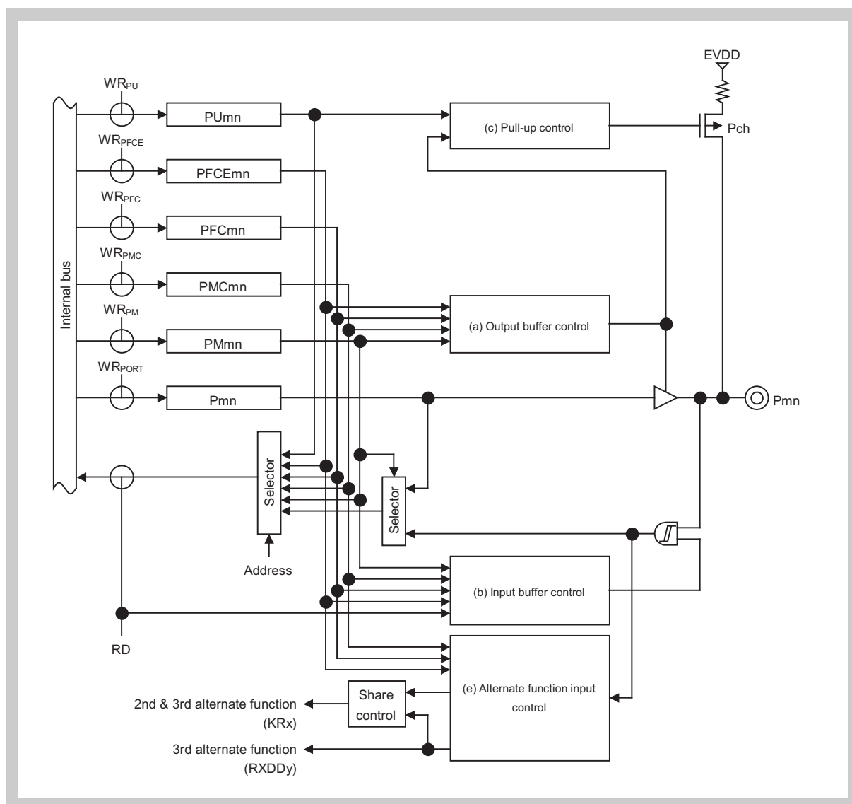
Figure 2-53 Port type Fx13x-U block diagram
