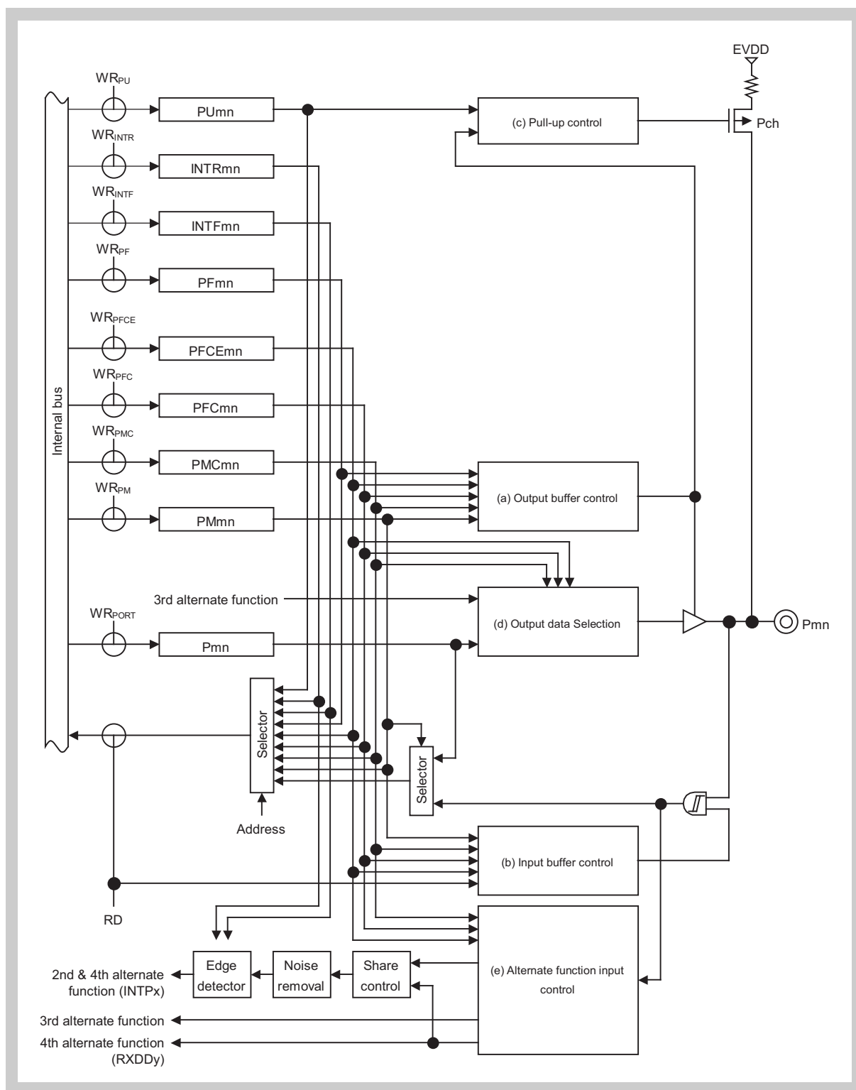
Figure 2-51 Port type Fx123-UF1 block diagram
