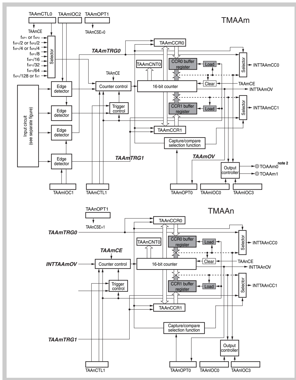
Figure 11-36 Block Diagram of TAAm and TAAm in 32-bit Capture Mode
