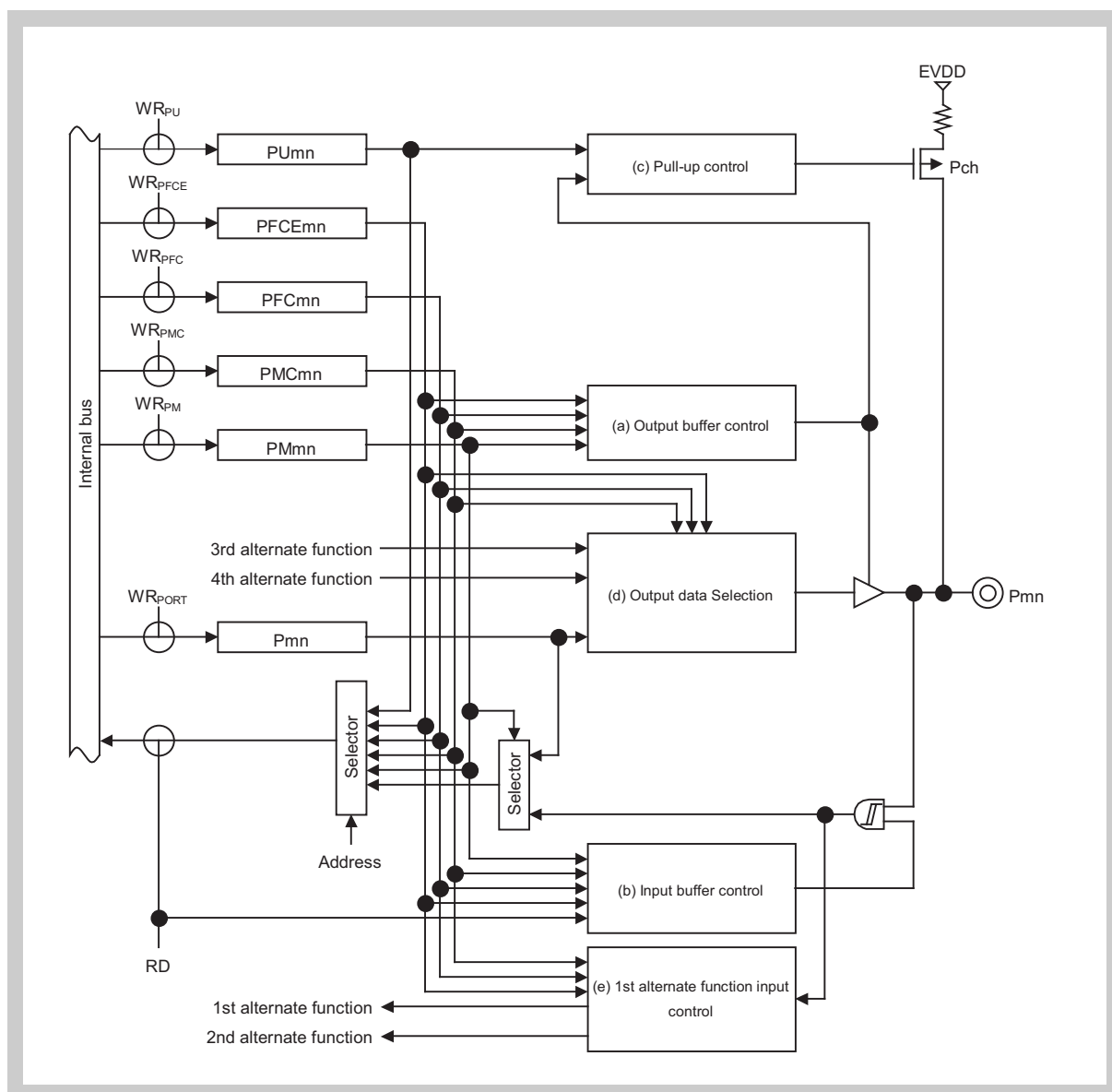
Figure 2-38 Port type F1100-U block diagram
