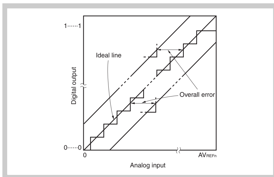
Figure 21-14 Overall error
