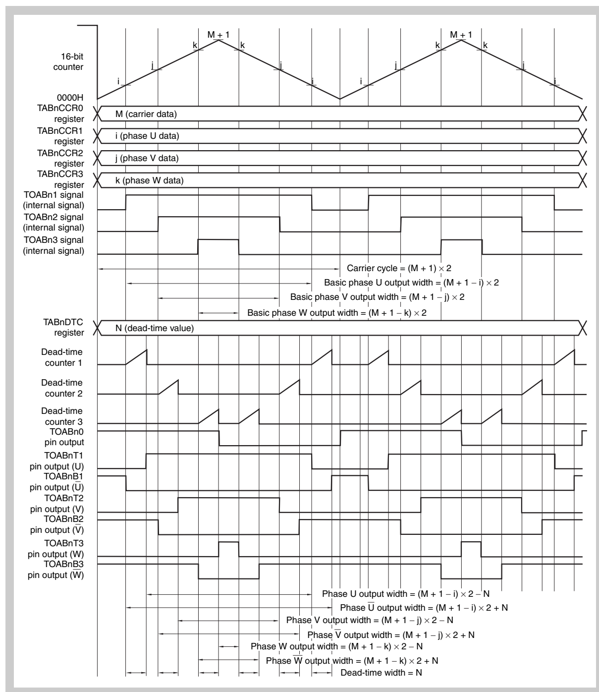
Figure 22-6 Timing Chart of 6-Phase PWM Output Mode
