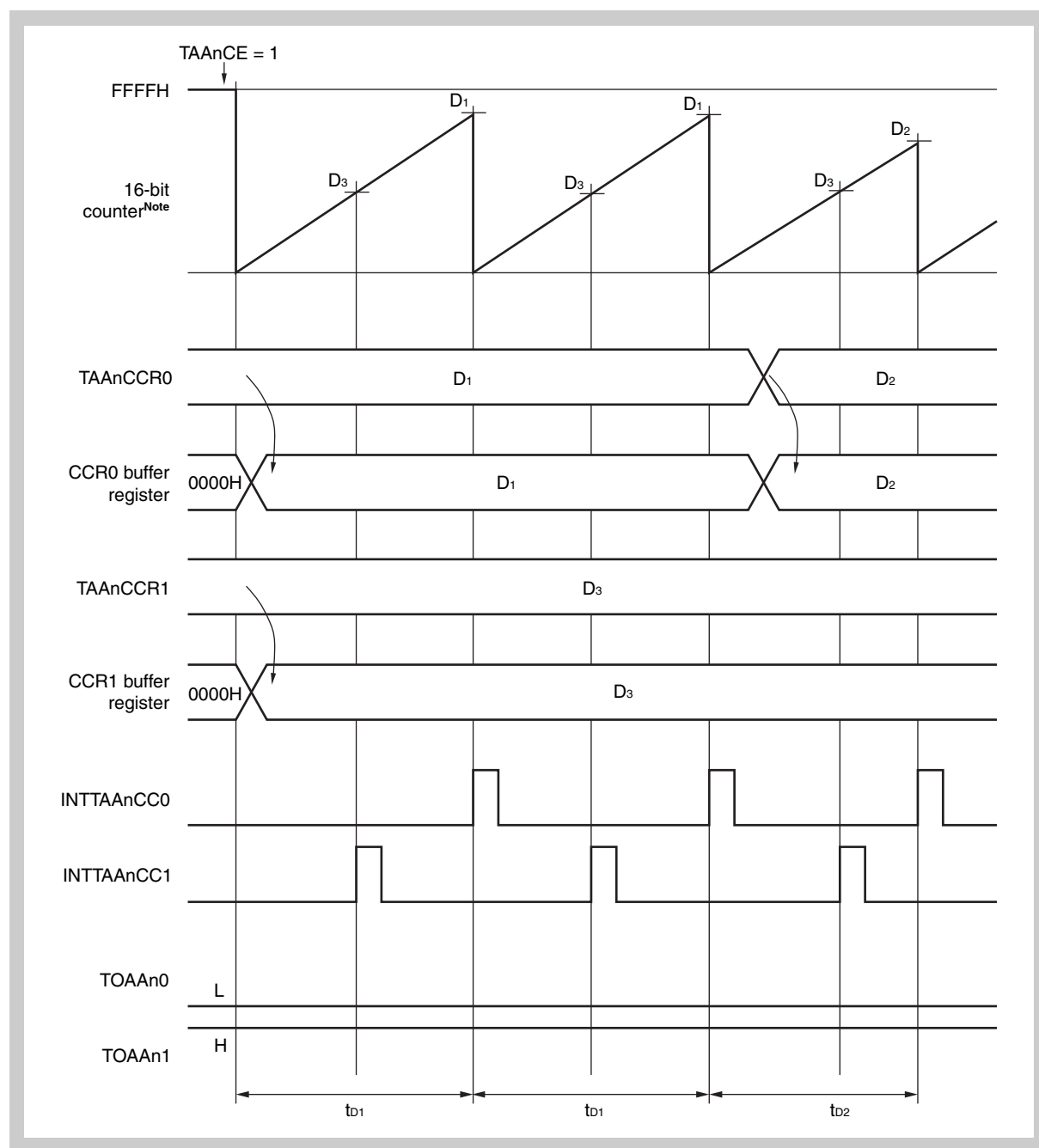
Figure 11-11 Basic operation timing in interval timer mode when D1 > D2 > D3 ; only TAAAnCCR0 register value is written, and TOAAAn0 and TOAAAn1 are not output (TAAAnOE0 = 0, TAAAnOE1 = 0, TAAAnOL0 = 0, TAAAnOL1 = 1)
