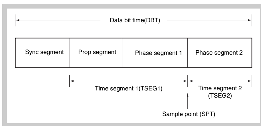
Figure 20-18 Segment setting
