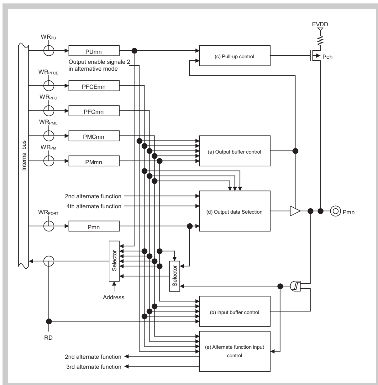
Figure 2-54 Port type Fx210-U block diagram
