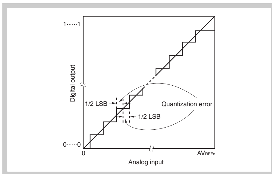
Figure 21-15 Quantization error
