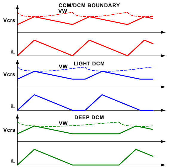
FIGURE 7. PERIOD STRETCHING
