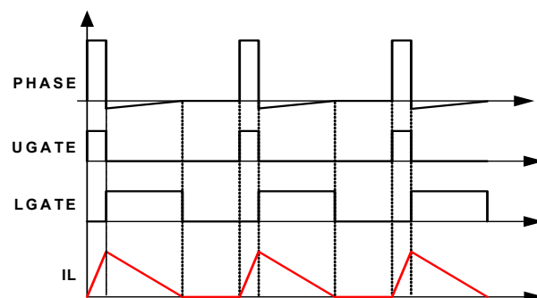
FIGURE 6. DIODE EMULATION
