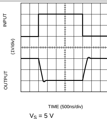
Figure 26. Inverting Large Signal Pulse Response
