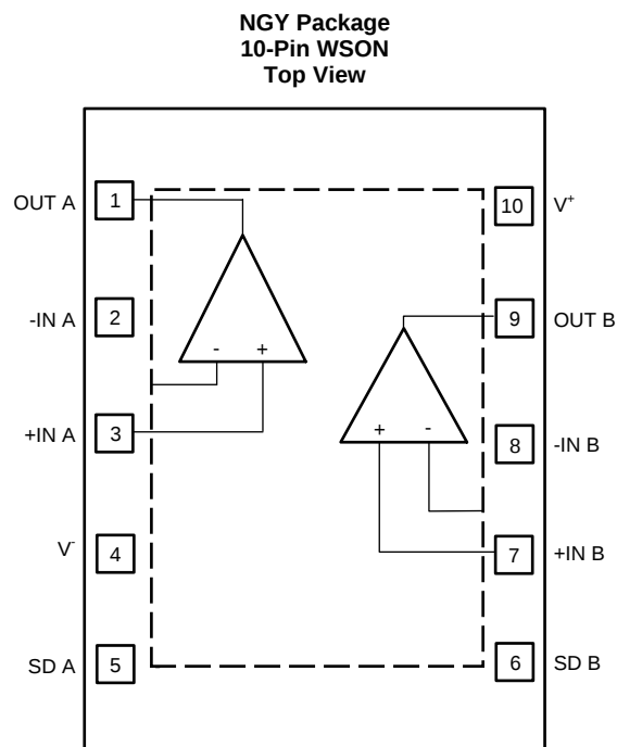
Pin Functions: WSON Package
