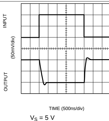
Figure 28. Inverting Small Signal Pulse Response
