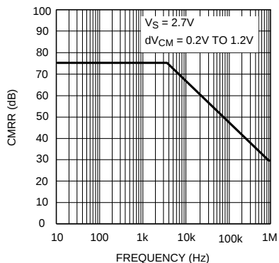
Figure 13. CMRR vs Frequency
