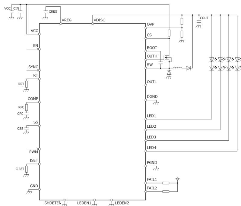
Figure 15. Buck Application Circuit
