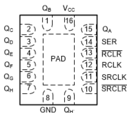
BQB or WBQB Package, 16-Pin WQFN (Top View)
