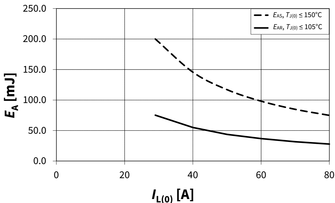
Figure 6 Maximum energy dissipation for inductive switch off, E_{AS/AR} vs. I_L at V_S = 13.5\text{ V}
