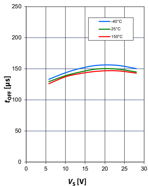
Turn OFF time
