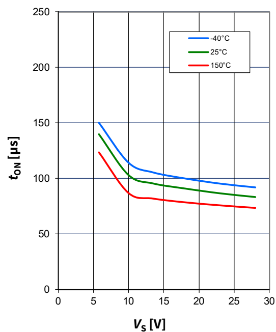
Turn ON time
