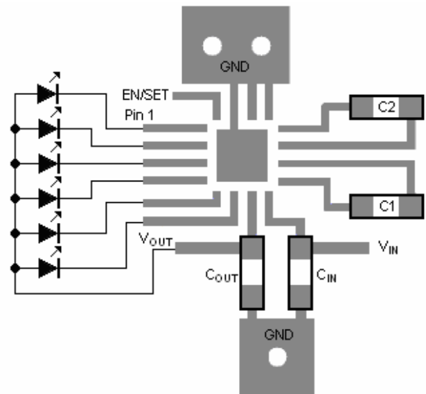
Figure 4. Recommended layout
