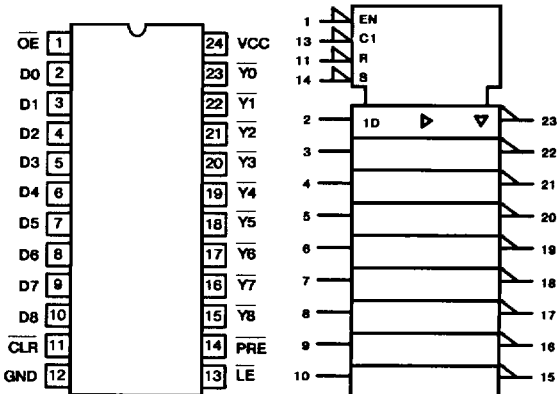
TERMINAL ASSIGNMENT
