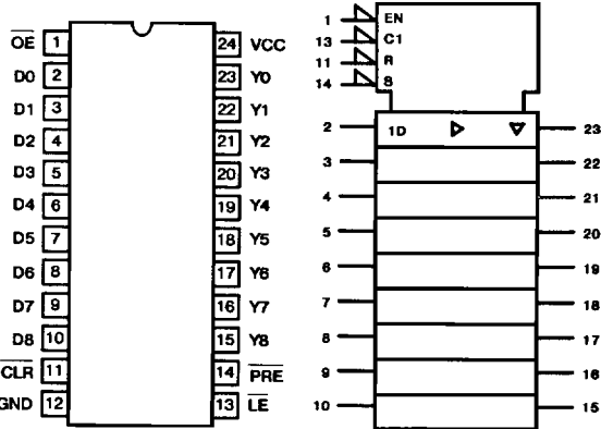
TERMINAL ASSIGNMENT
