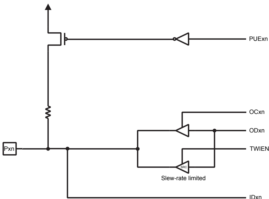
Figure 27-7. Additional Scan Signal for the Two-wire Interface
