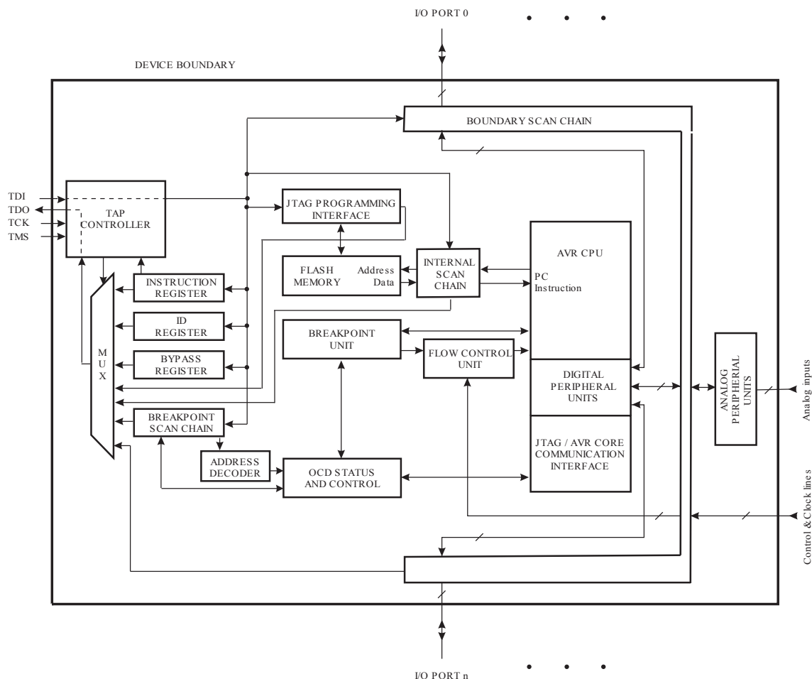
Figure 27-1. Block Diagram
