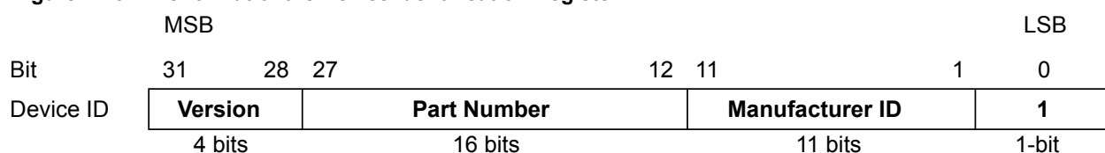
Figure 27-3. The format of the Device Identification Register
