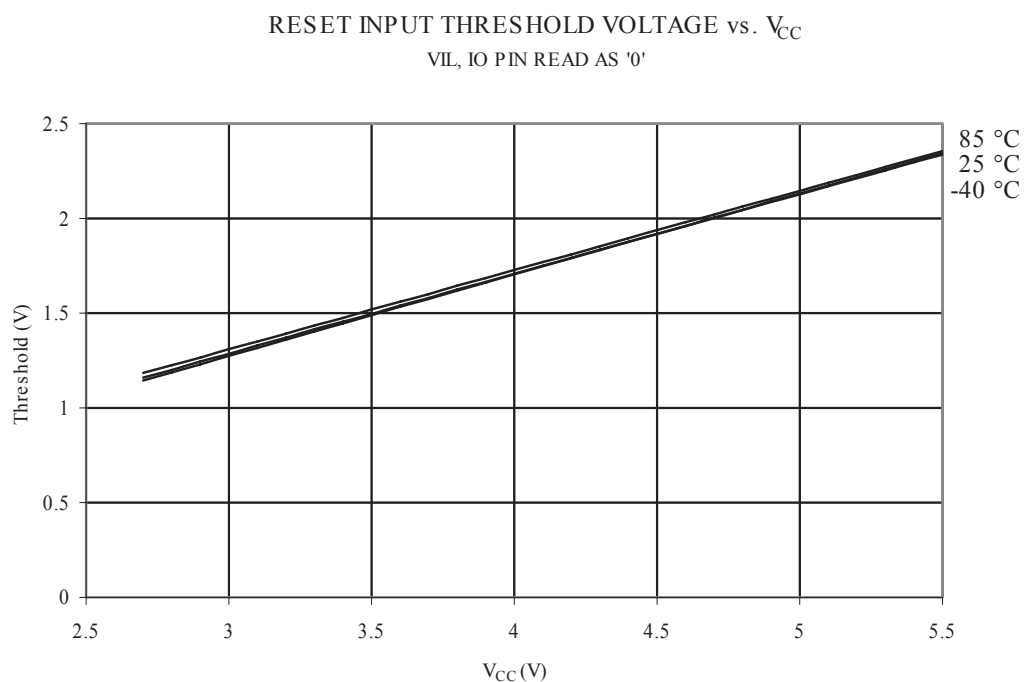
Figure 31-29. Reset Input Threshold Voltage vs. V_{CC} ( V_{IL} , Reset Pin Read as “0”)
