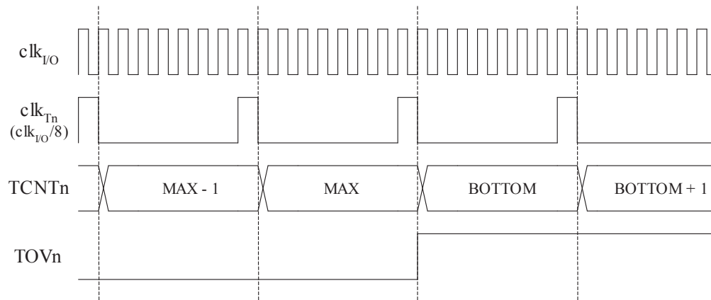
Figure 20-9. Timer/Counter Timing Diagram, with Prescaler ( f_{\text{clk}_{I/O}/8} )
