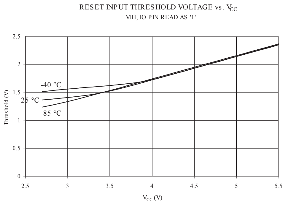
Figure 31-28. Reset Input Threshold Voltage vs. V_{CC} ( V_{IH} , Reset Pin Read as “1”)
