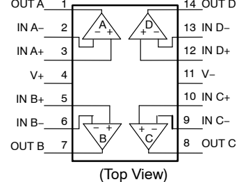
TSSOP-14
