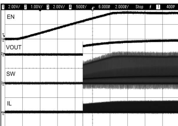
Figure 30. Cold-Start Transient Response from 0 mA to 100 mA
