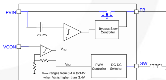
Figure 36. Enabling Bypass Transistor Circuit
