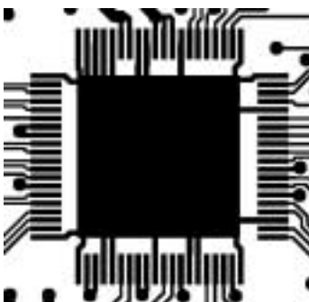
Figure 10. Example of a Thermal Land for the TSB41LV04A PHY
